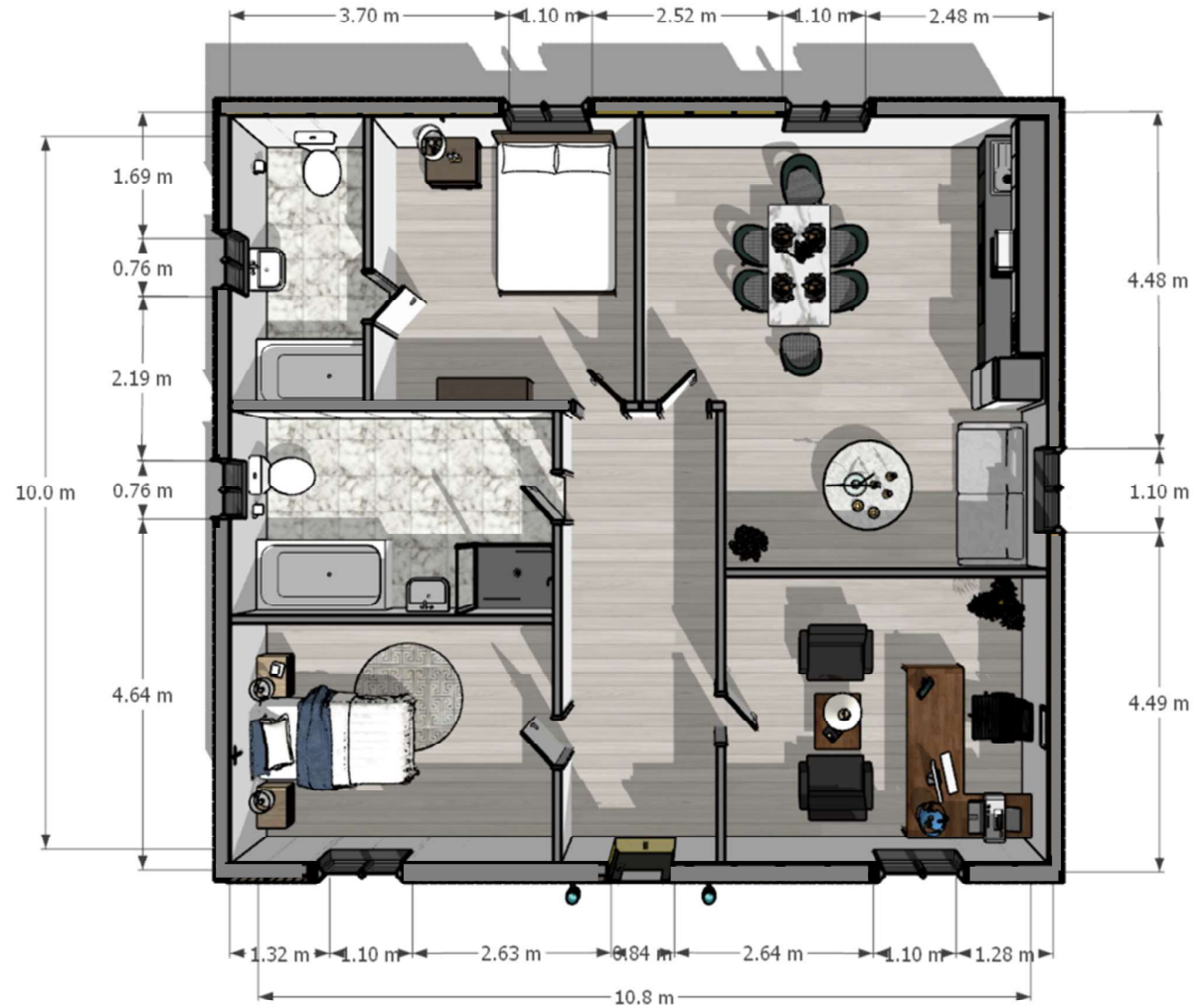
FLOOR PLAN 02 – FURNITURE LAYOUT & EXTERNAL DIMENSIONS
