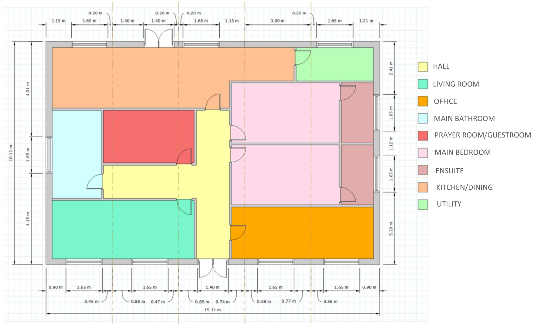
FLOOR PLAN 04 – MODULE DIMENSIONS
