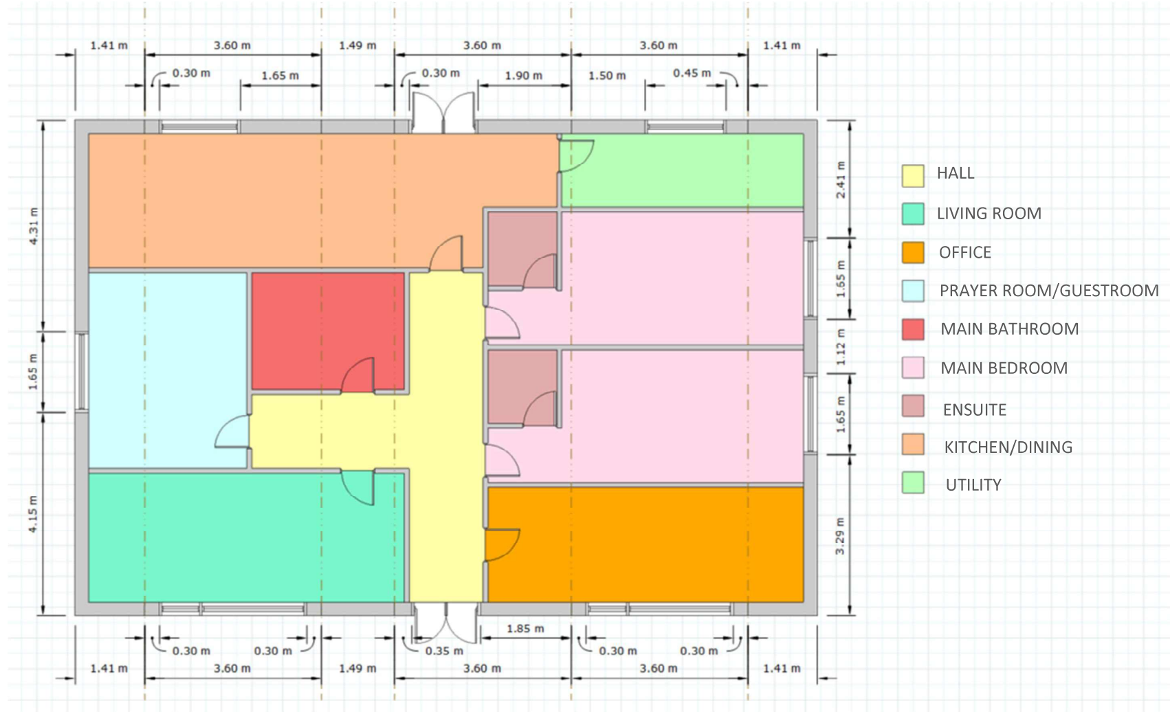
FLOOR PLAN 04 – MODULE DIMENSIONS
