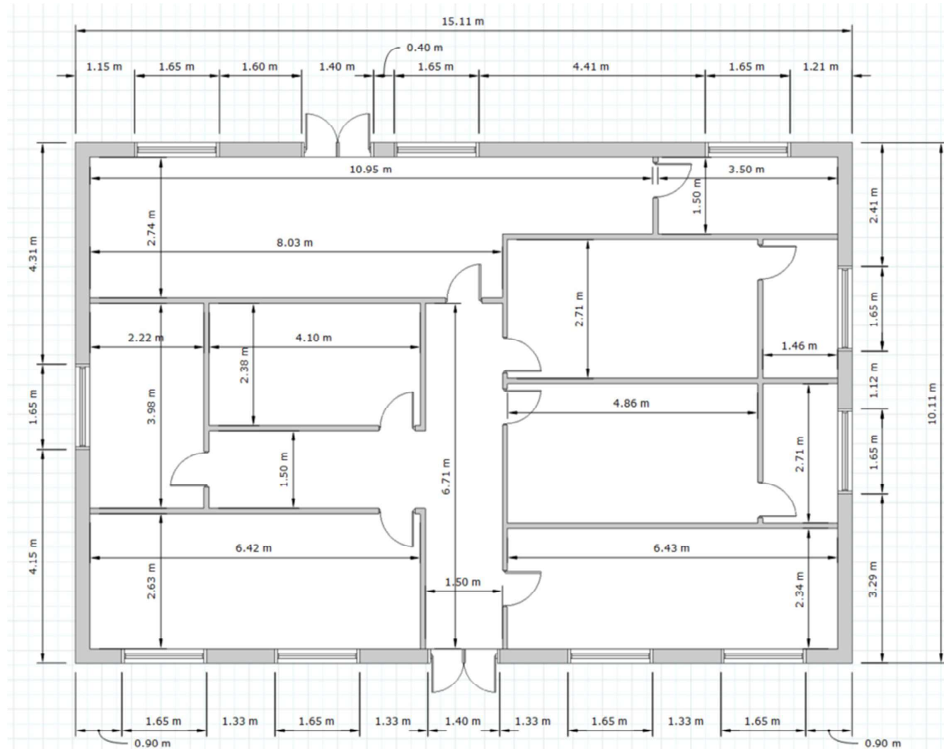
FLOOR PLAN 03 – EXTERNAL & INTERNAL DIMENSIONS
