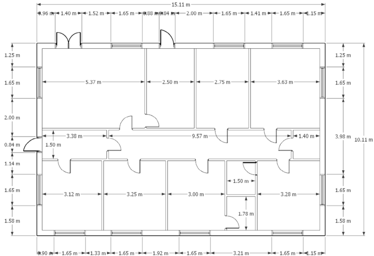
FLOOR PLAN 03 – EXTERNAL & INTERNAL DIMENSIONS
