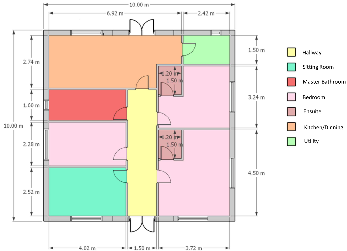
FLOOR PLAN 01
