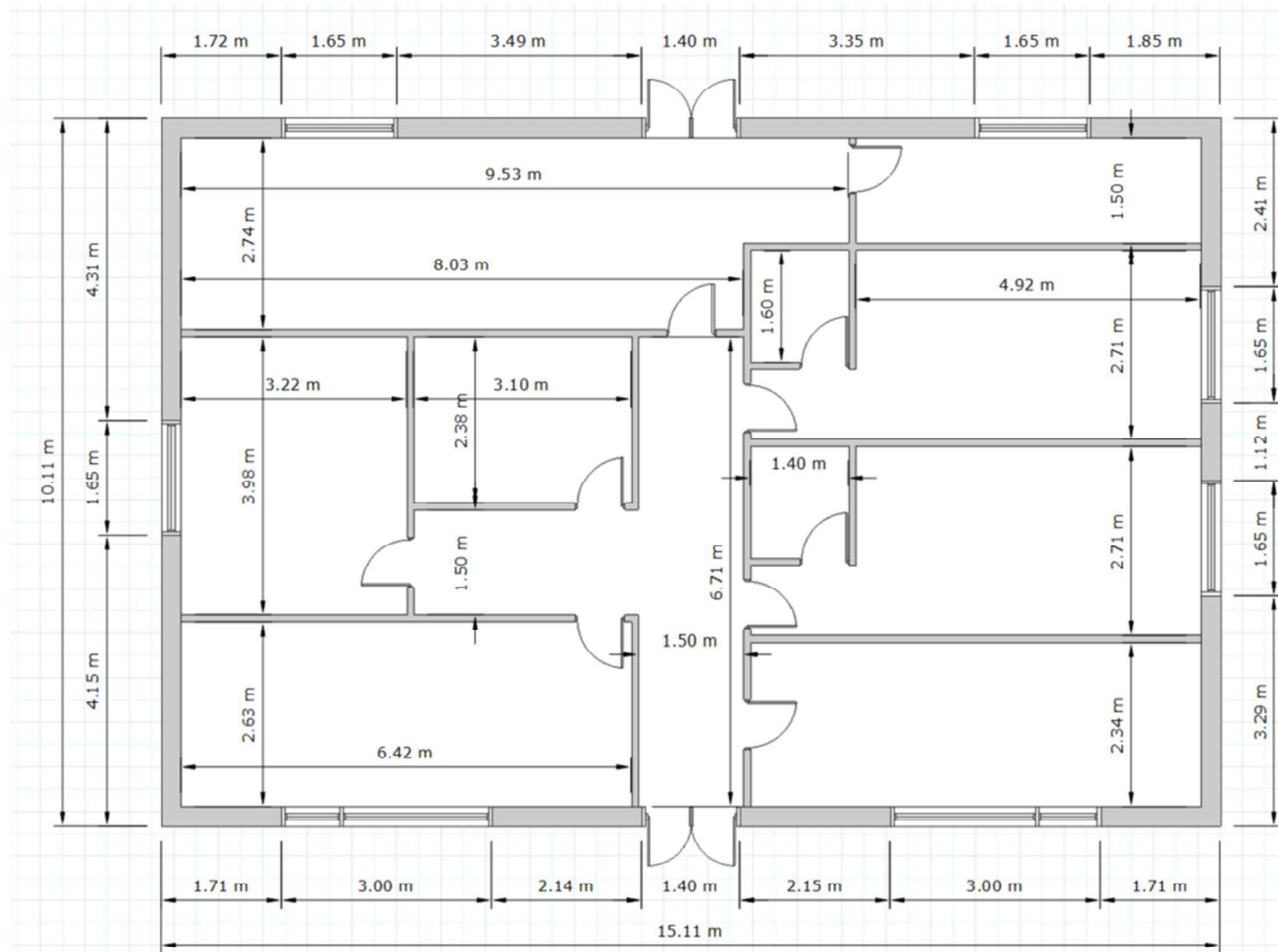
FLOOR PLAN 03 – EXTERNAL &amp; INTERNAL DIMENSIONS
