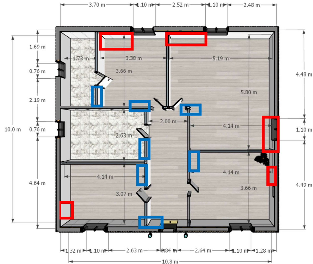
FLOOR PLAN 01 – SOCKET & SWITCHES
