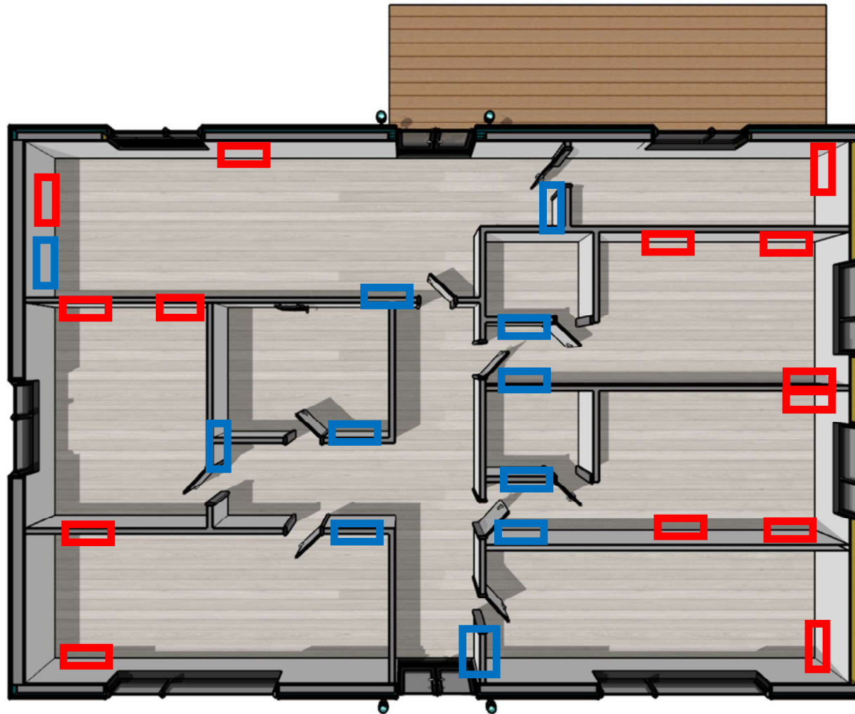
FLOOR PLAN 01 – SOCKET & SWITCHES
