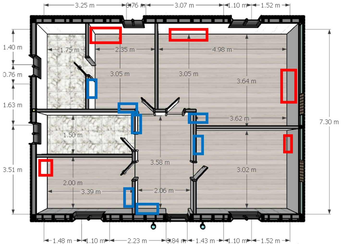
FLOOR PLAN 01 – SOCKET & SWITCHES
