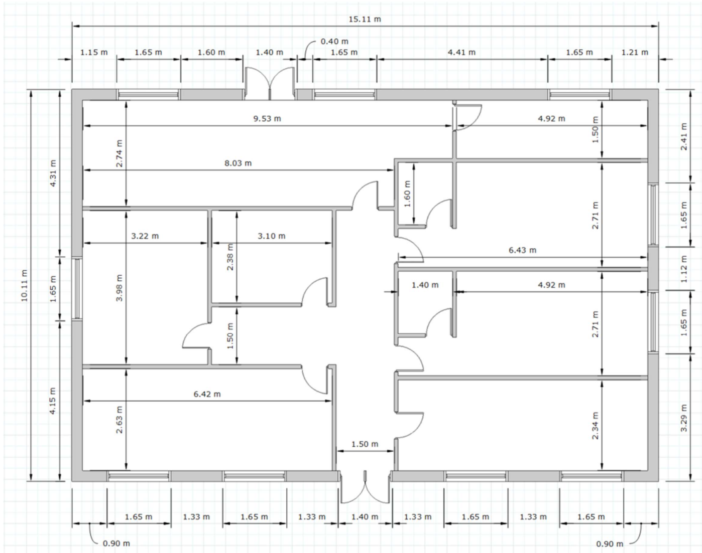
FLOOR PLAN 03 – EXTERNAL & INTERNAL DIMENSIONS
