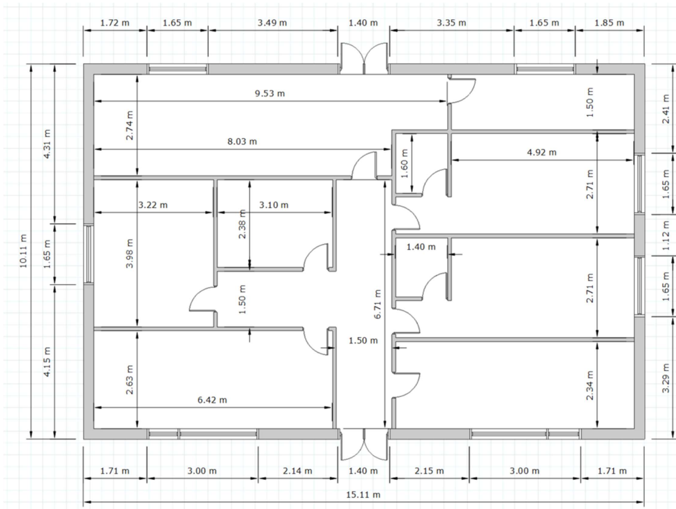
FLOOR PLAN 03 – EXTERNAL & INTERNAL DIMENSIONS
