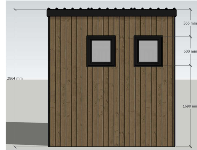
REAR ELEVATION W/ DIMENSIONS
