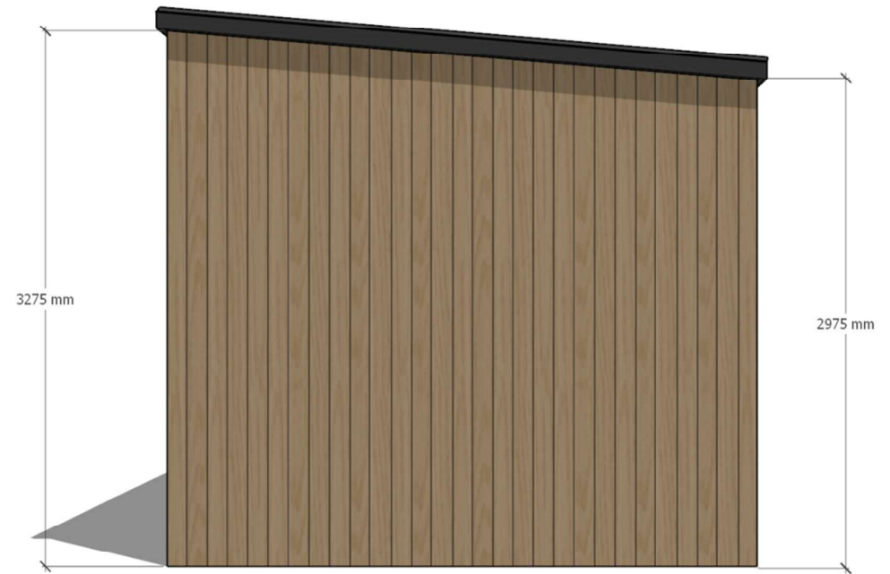
RHS ELEVATION W/ DIMESNIONS
