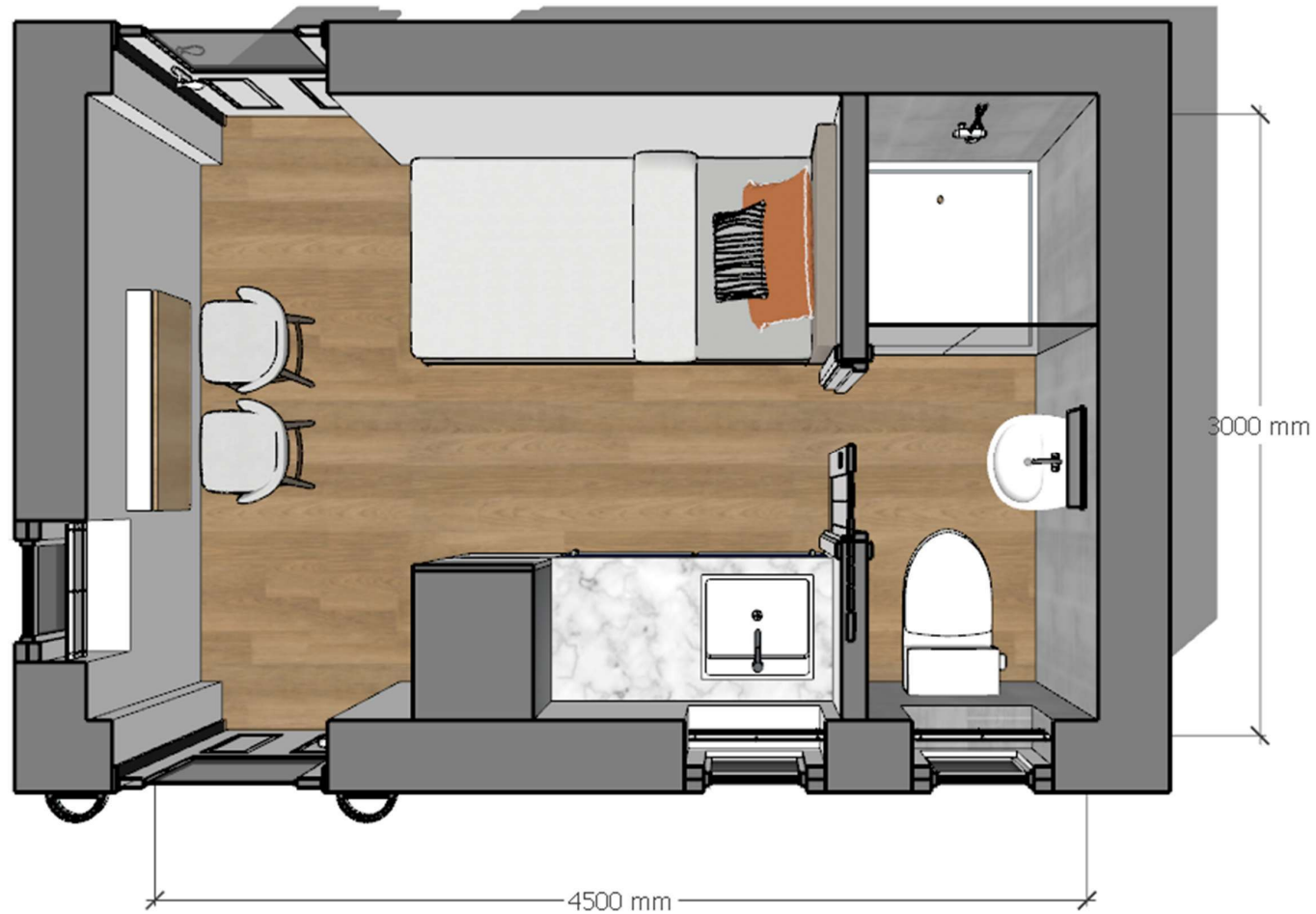
FLOOR PLAN 02 – FURNITURE LAYOUT (EXAMPLE ONLY)
