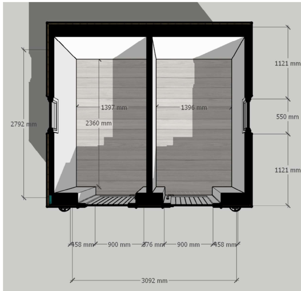
FLOOR PLAN 02 – EXTERNAL & INTERNAL DIMENSIONS
