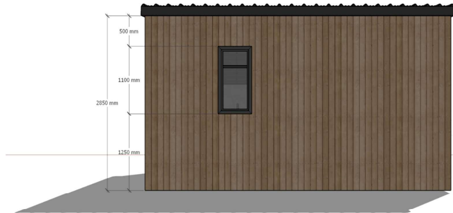
REAR ELEVATION W/ DIMENSIONS
