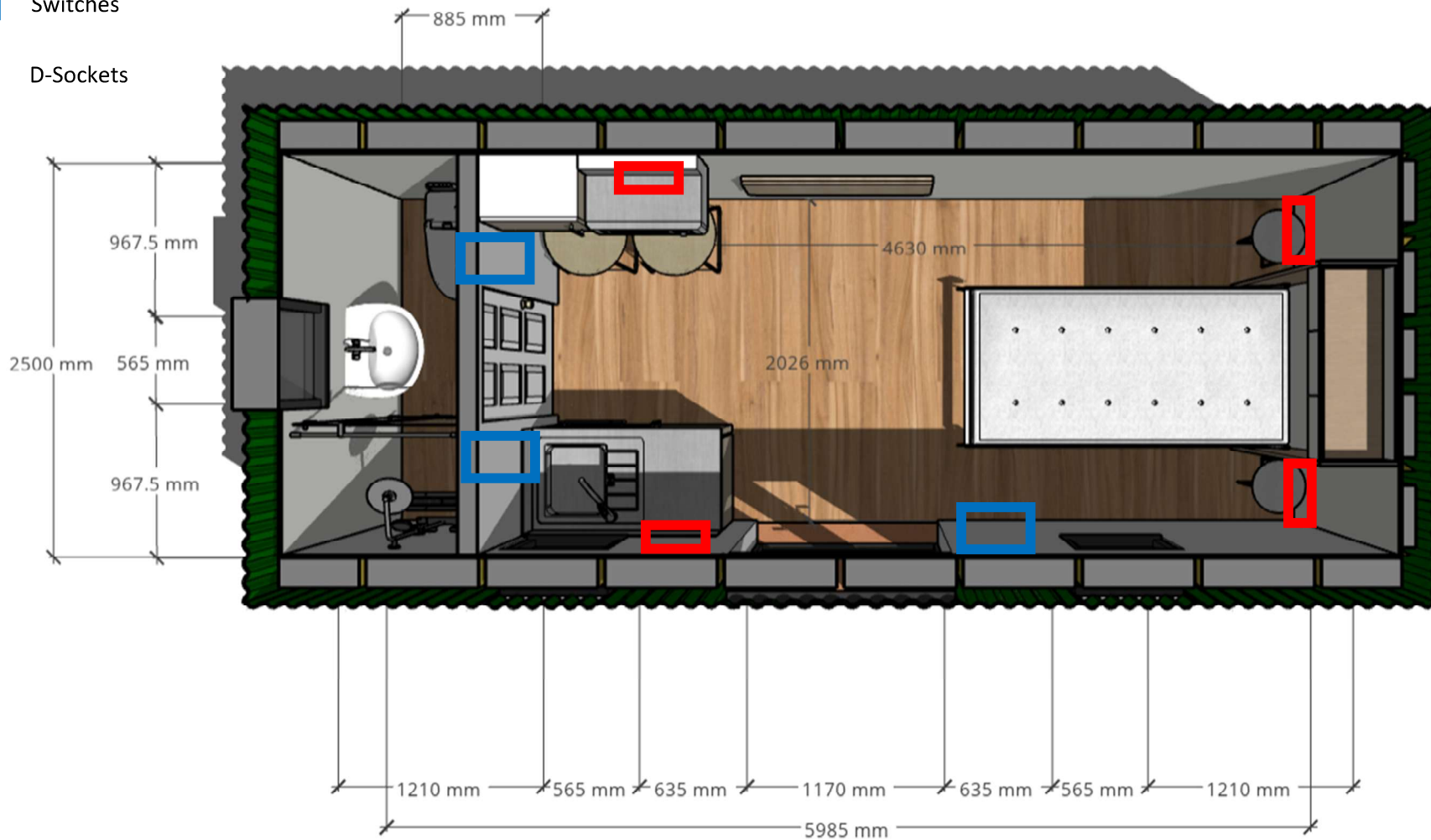
FLOOR PLAN 02
