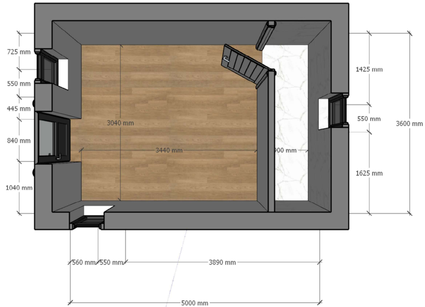
FLOOR PLAN 02 – EXTERNAL & INTERNAL DIMENSIONS
