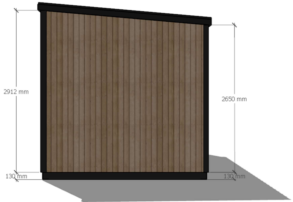
RHS ELEVATION W/ DIMENSIONS
