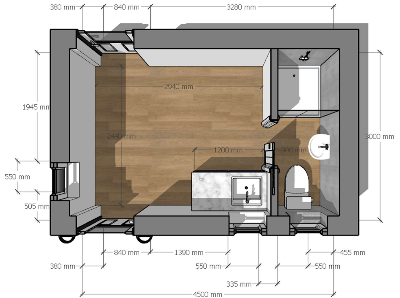
FLOOR PLAN 01 –LAYOUT
