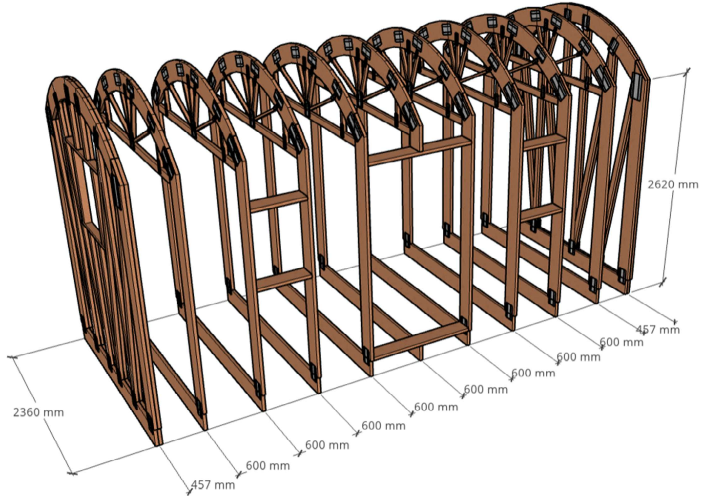
PROPOSED FRAME SETTING OUT
