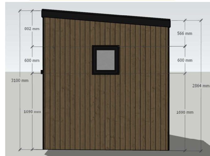
RHS ELEVATION W/ DIMENSIONS
