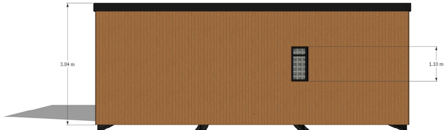
REAR ELEVATION
