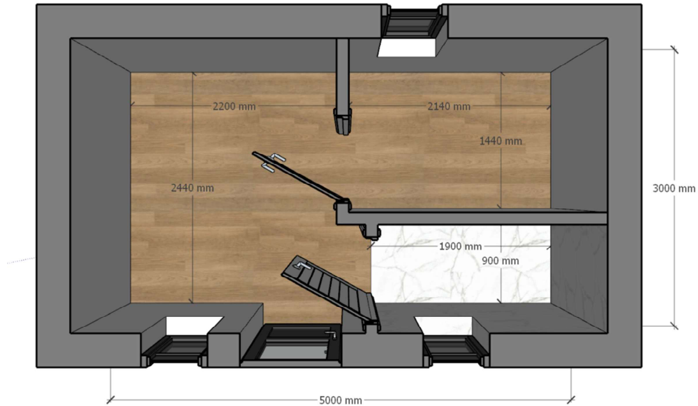
FLOOR PLAN 03 – EXTERNAL & INTERNAL DIMENSIONS
