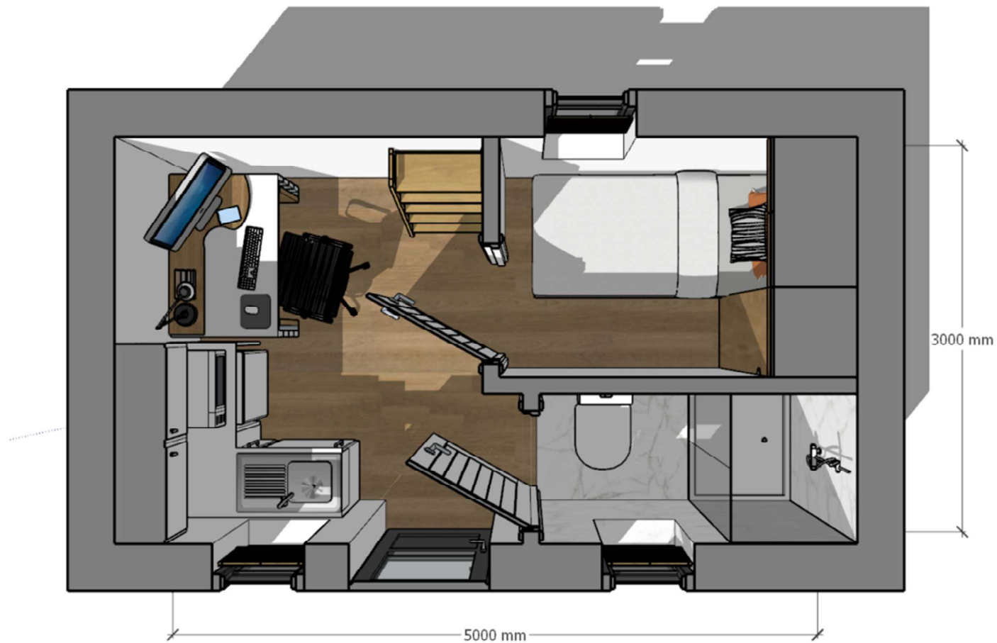
FLOOR PLAN 02 – FURNITURE LAYOUT (EXAMPLE ONLY)
