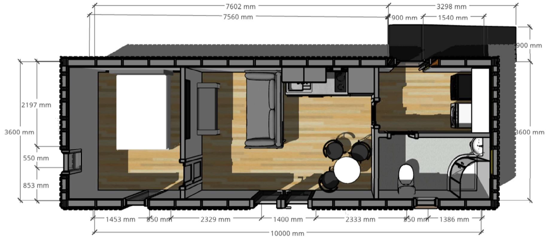
FLOOR PLAN 02
