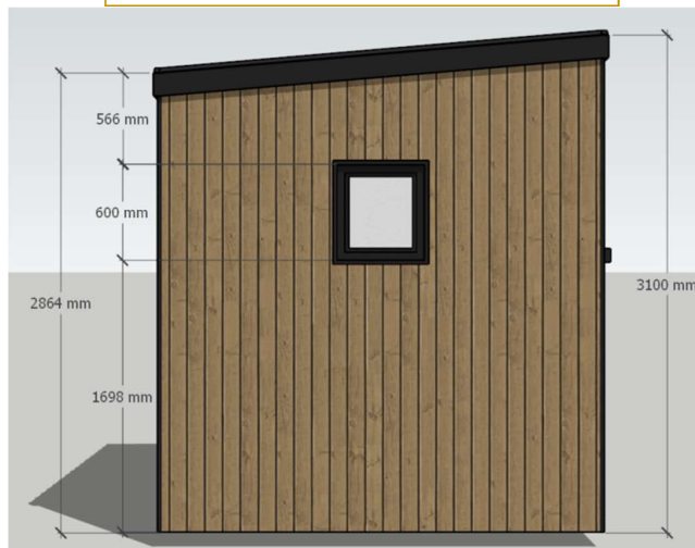
LHS ELEVATION W/ DIMENSIONS
