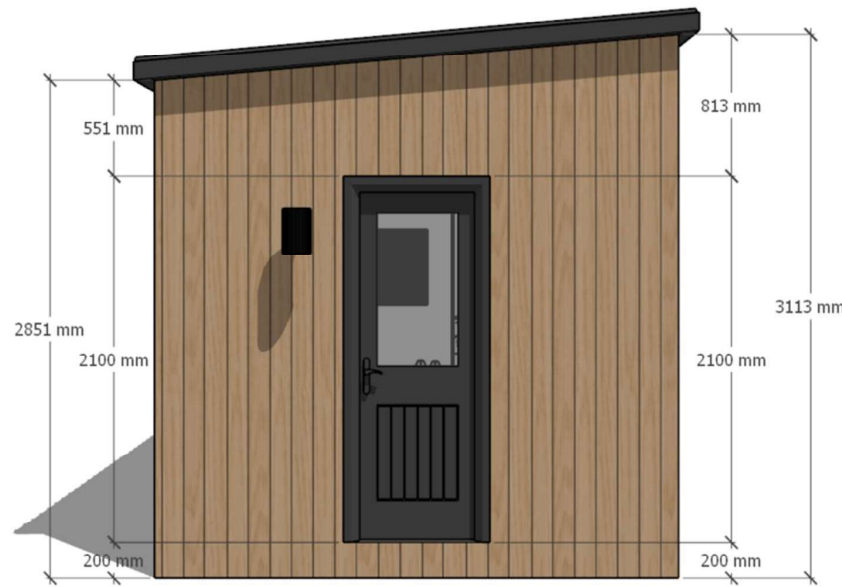
LHS ELEVATION
