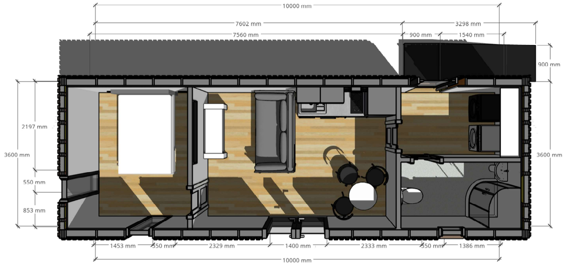
FLOOR PLAN 02
