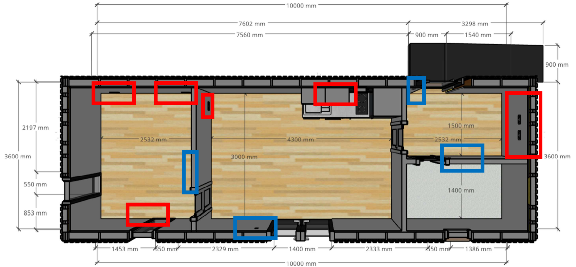
FLOOR PLAN 01
