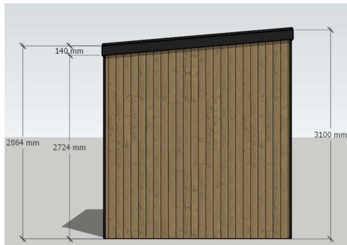
LHS ELEVATION W/ DIMENSIONS
