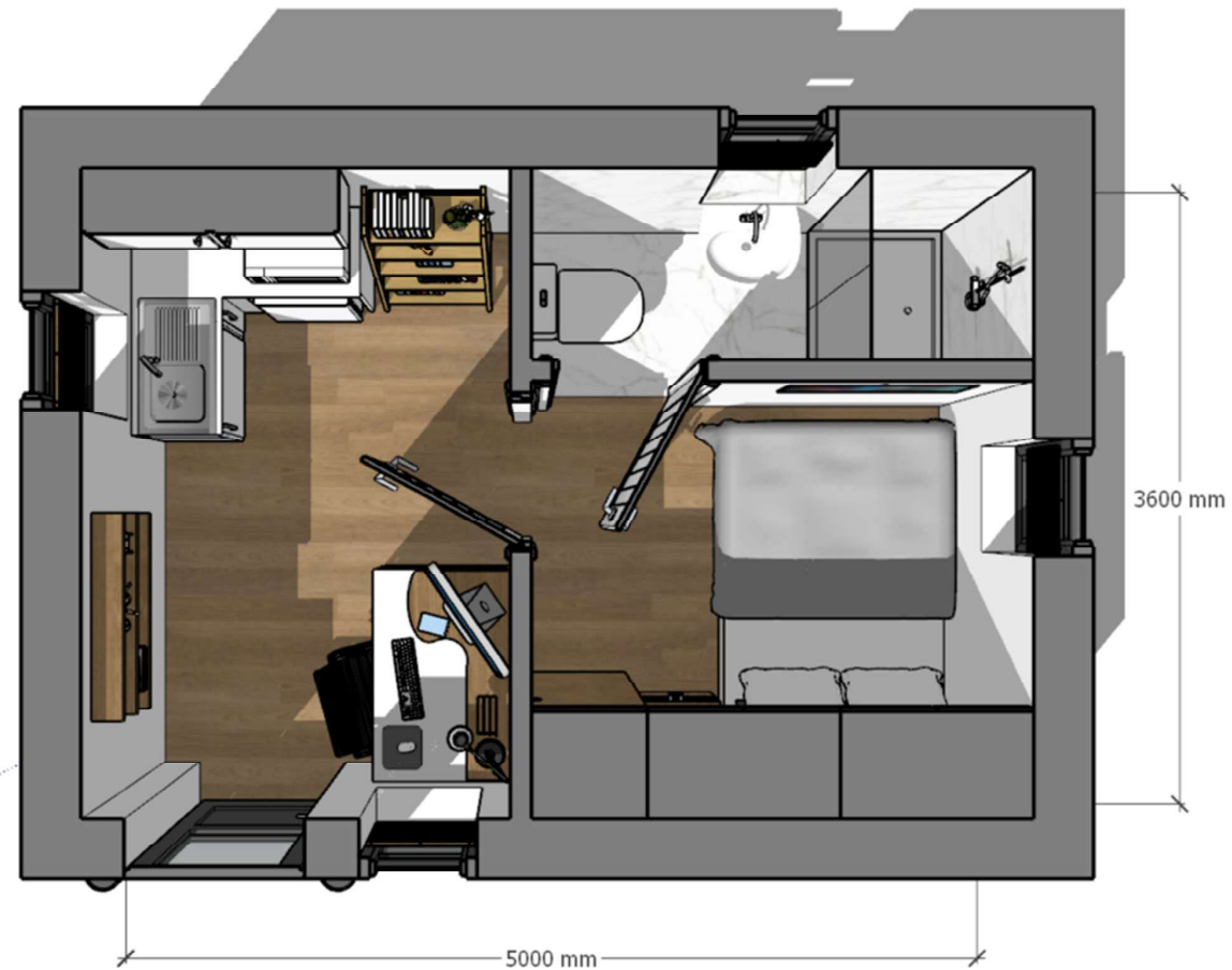
FLOOR PLAN 01 – FURNITURE LAYOUT (EXAMPLE ONLY)
