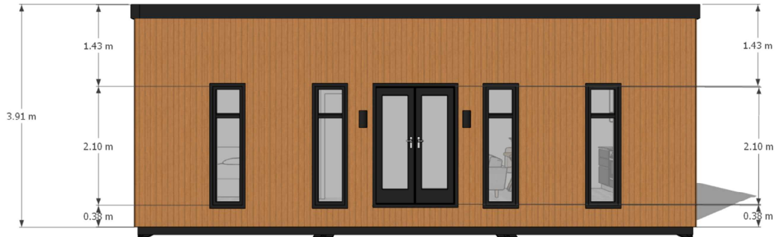
FRONT ELEVATION
