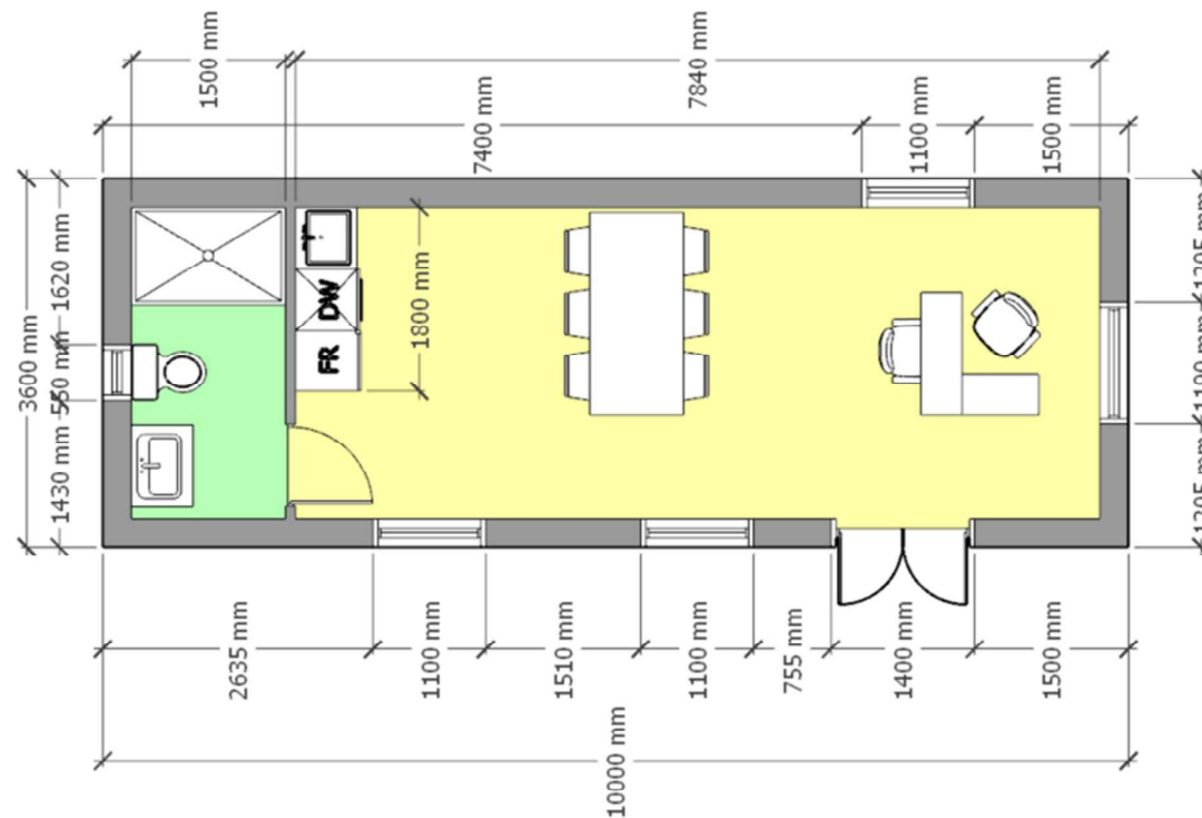
FLOOR PLAN 01
