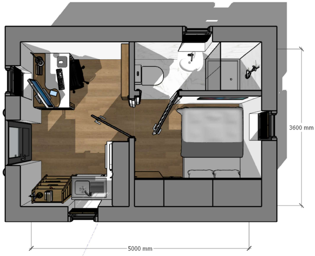
FLOOR PLAN 01 – FURNITURE LAYOUT (EXAMPLE ONLY)
