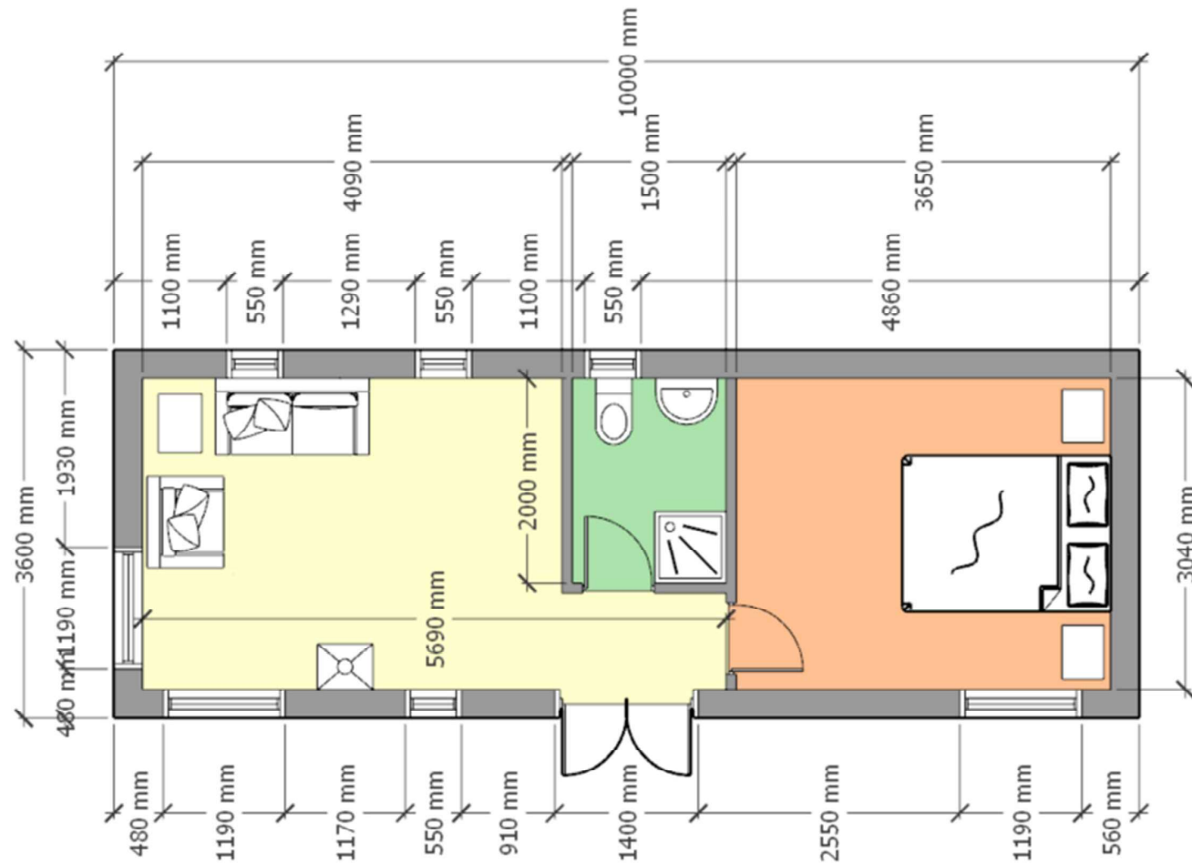
FLOOR PLAN 03 – EXTERNAL & INTERNAL DIMENSIONS
