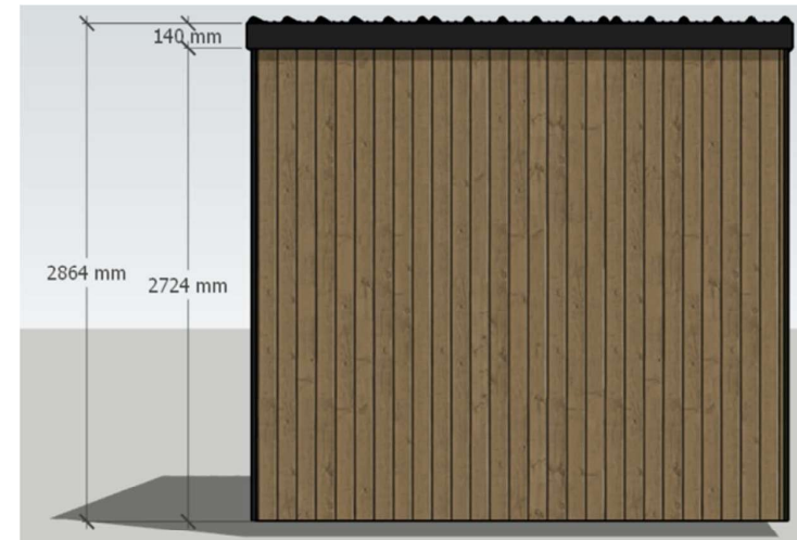
REAR ELEVATION W/ DIMENSIONS
