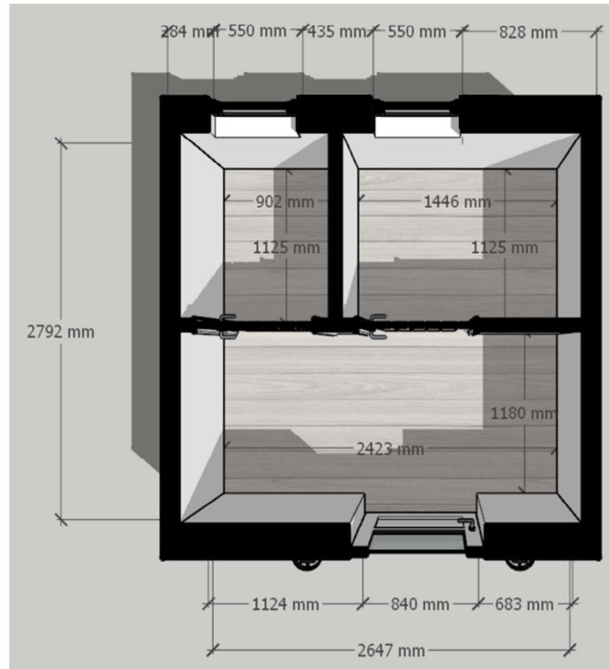
FLOOR PLAN 03 – EXTERNAL & INTERNAL DIMENSIONS
