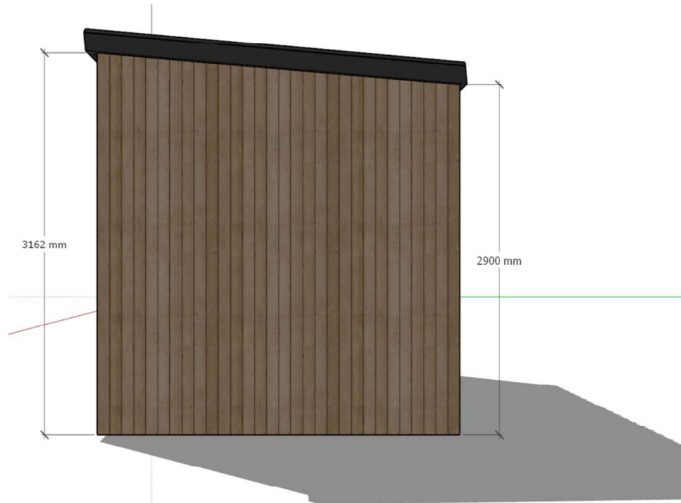
RHS ELEVATION W/ DIMENSIONS
