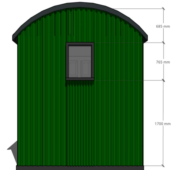
LHS ELEVATION
