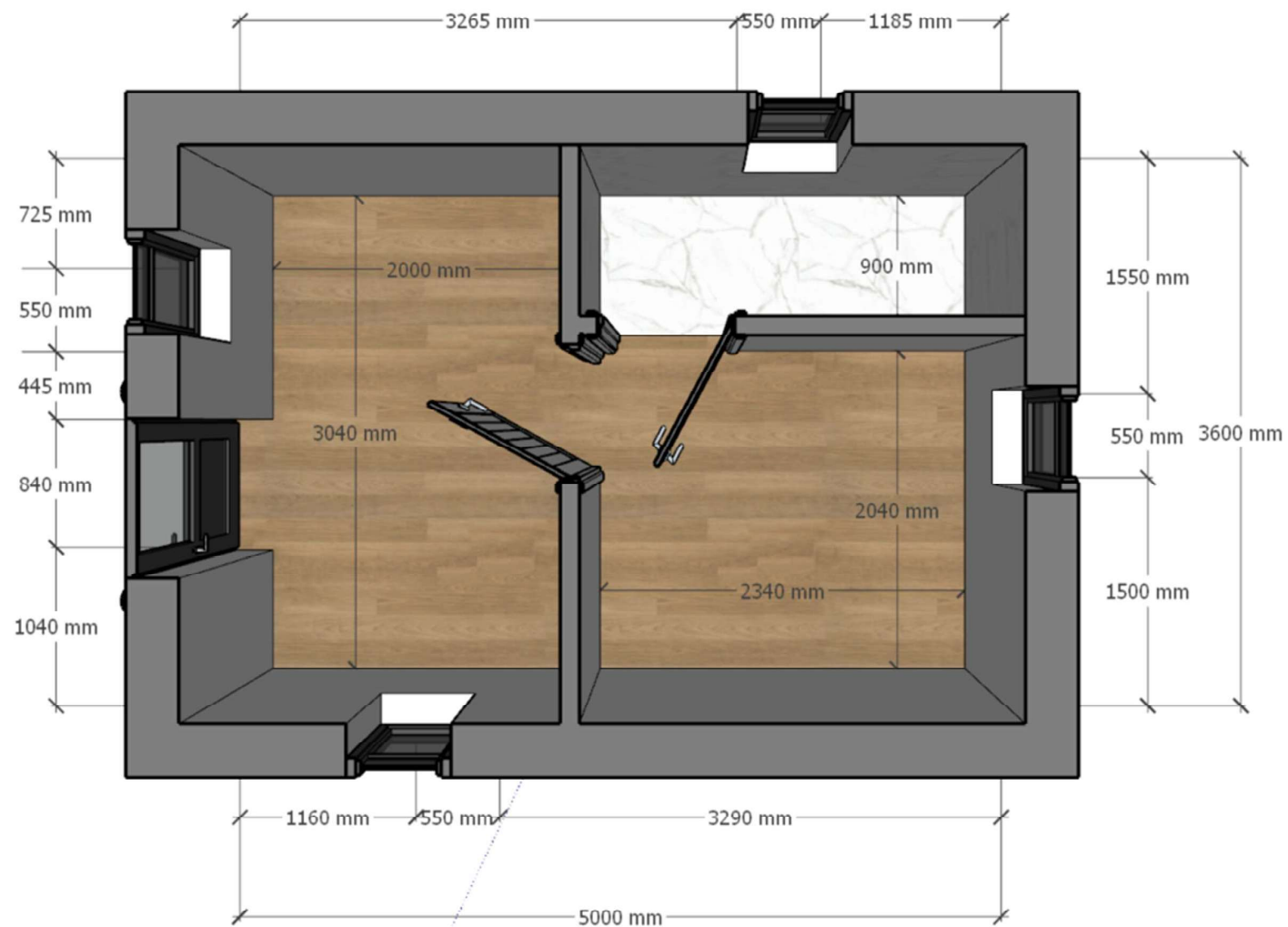
FLOOR PLAN 02 – EXTERNAL & INTERNAL DIMENSIONS
