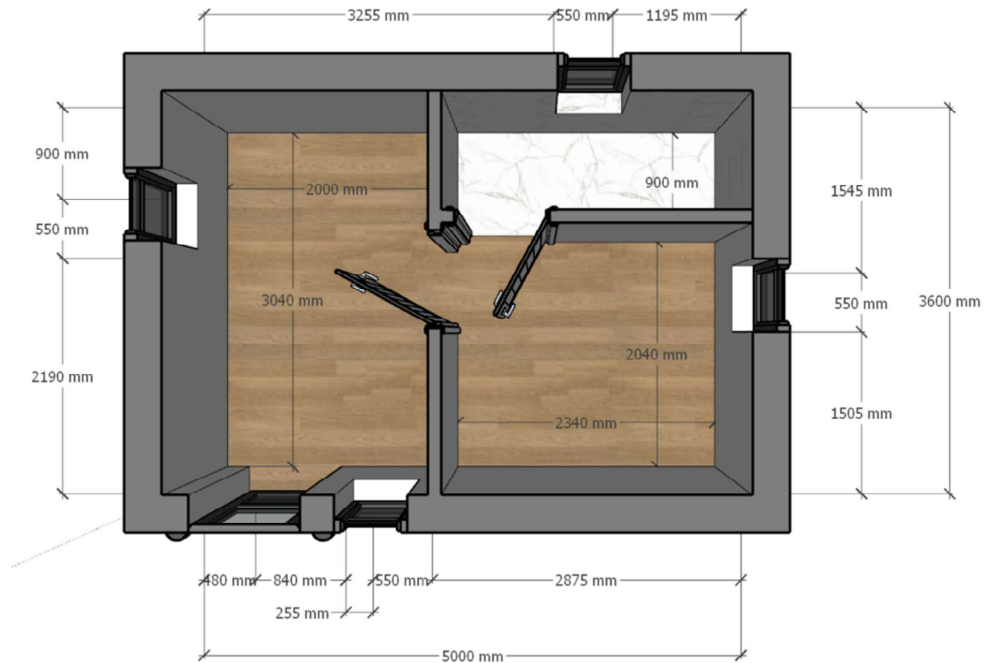
FLOOR PLAN 02 – EXTERNAL & INTERNAL DIMENSIONS
