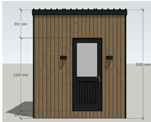
FRONT ELEVATION W/ DIMENSIONS
