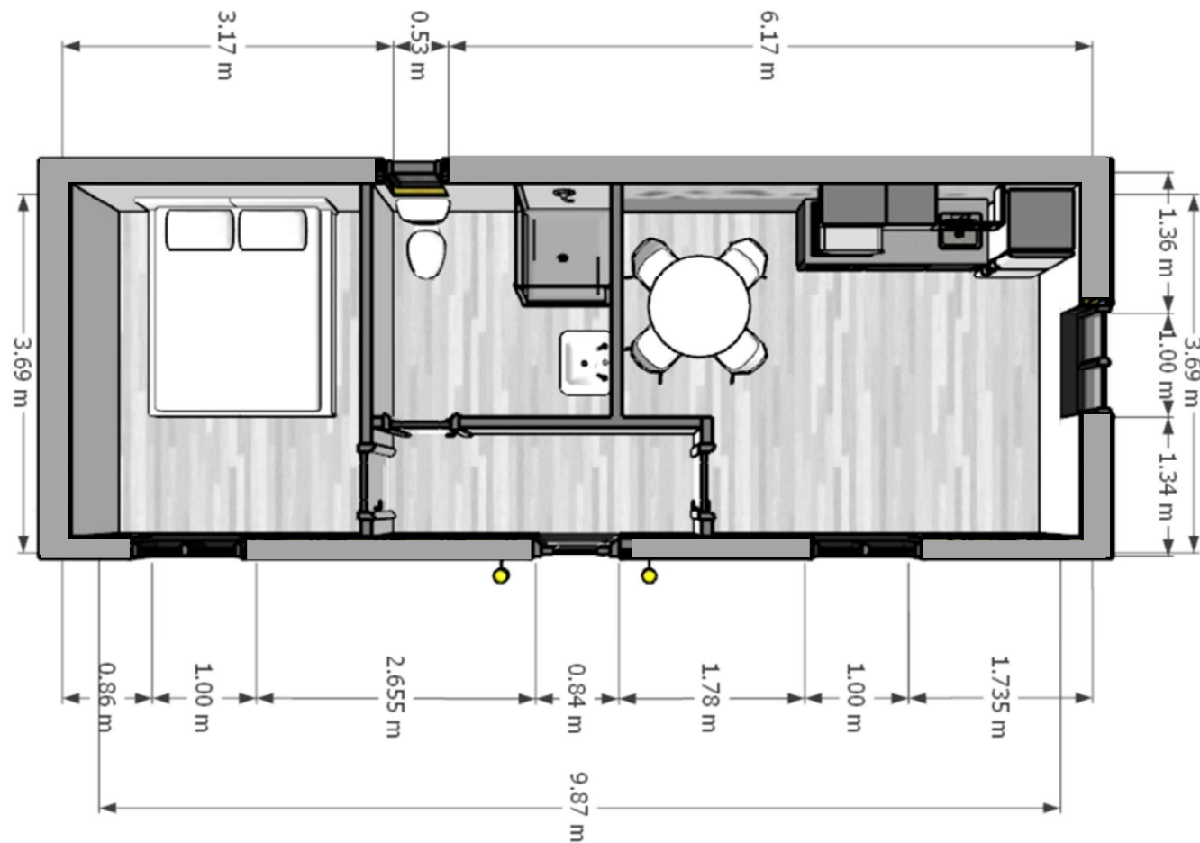
FLOOR PLAN 0 – FURNITURE LAYOUT & EXTERNAL DIMENSIONS
