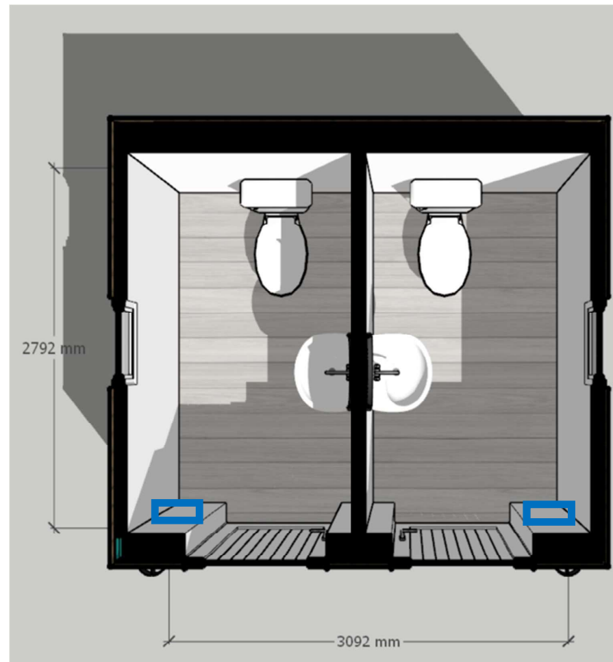
FLOOR PLAN 01 – SOCKET & SWITCHES
