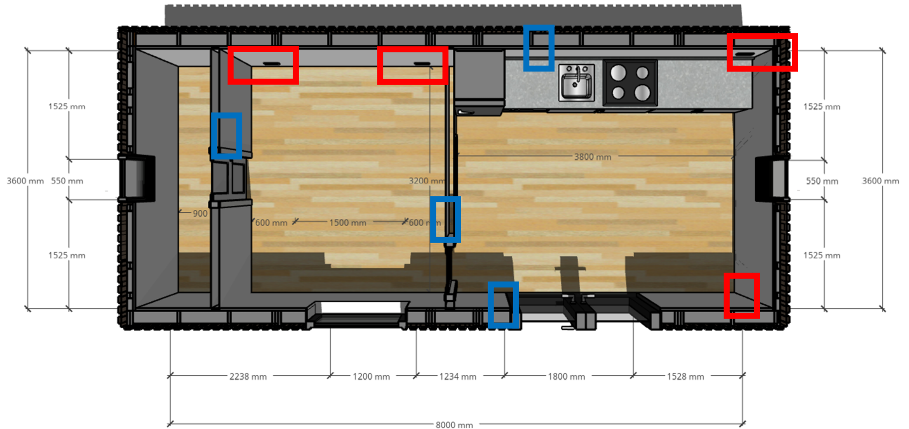
FLOOR PLAN 01
