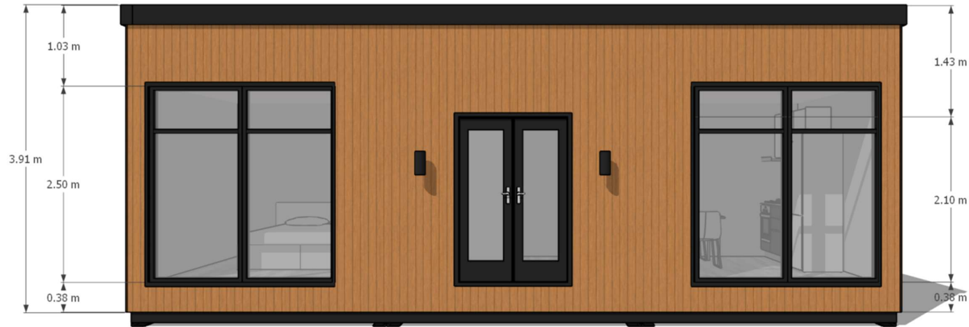
FRONT ELEVATION
