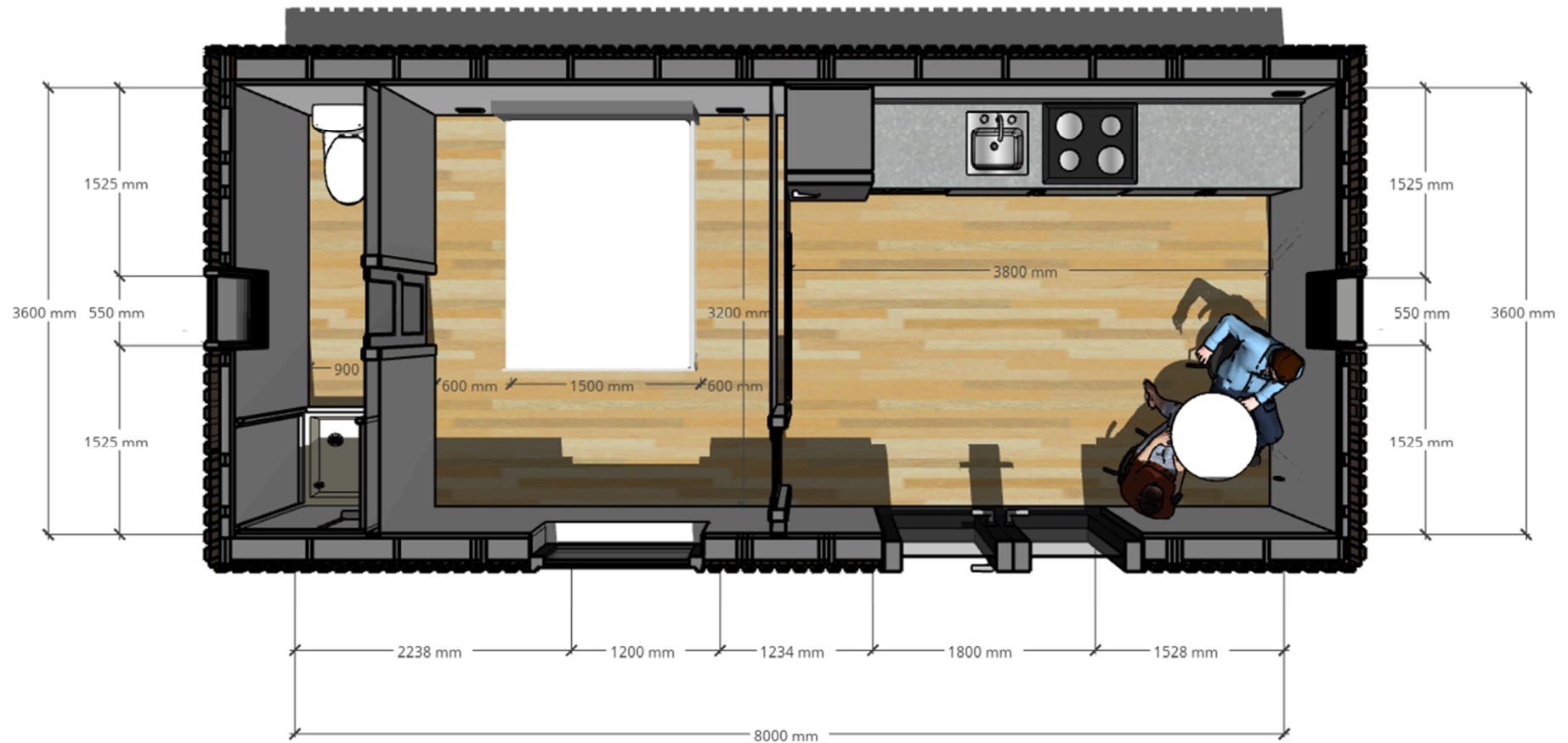
FLOOR PLAN 02
