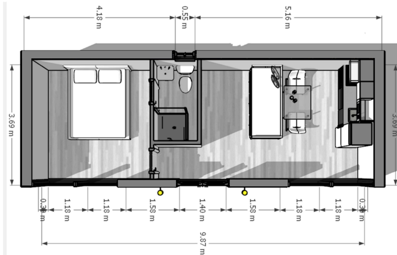
FLOOR PLAN 02 – FURNITURE LAYOUT & EXTERNAL DIMENSIONS
