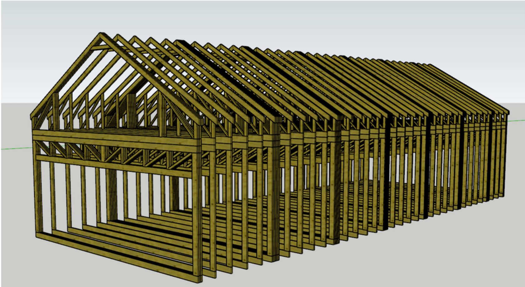
FRAME DESIGN – 2 STOREY
