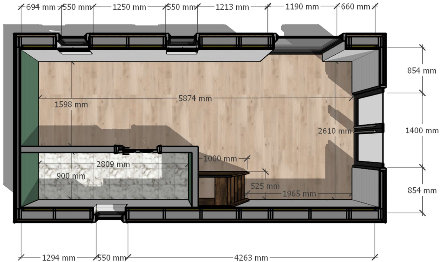
FLOOR PLAN 01 – INTERNAL DIMENSIONS
