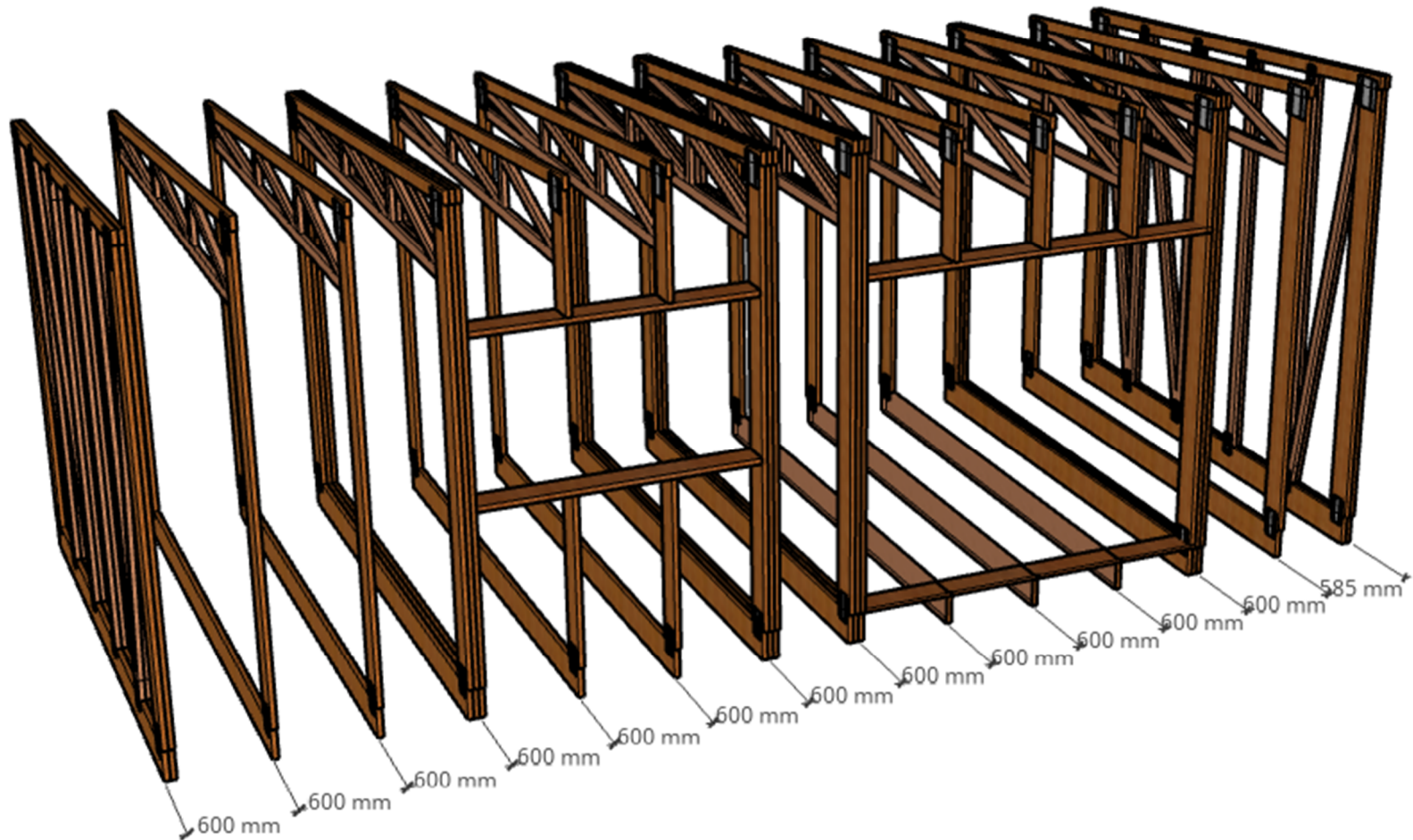
Frame set out
