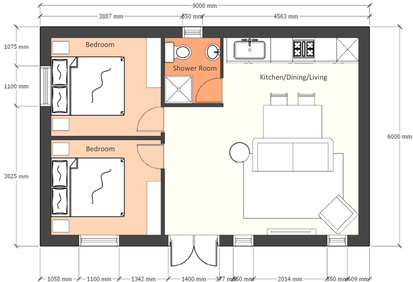
FLOOR PLAN 01
