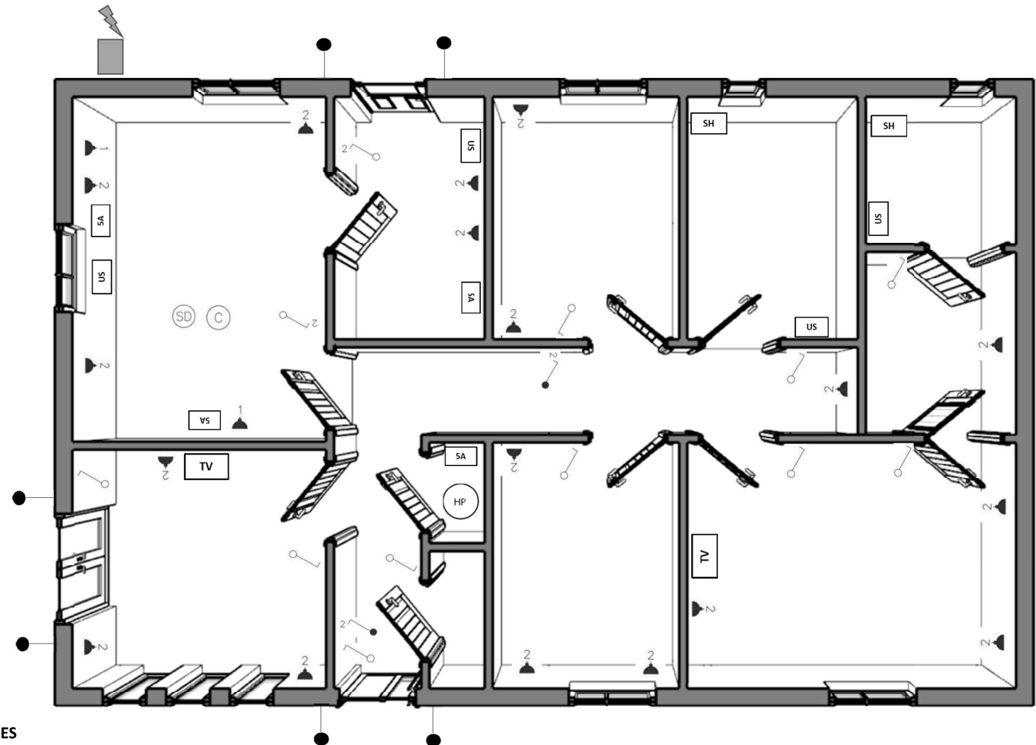
ELECTRICAL LAYOUT
