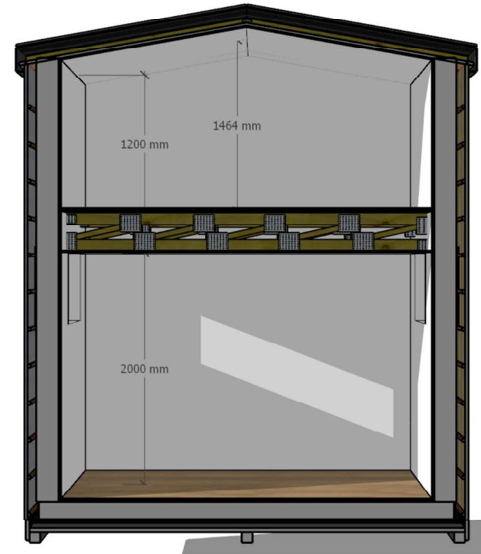
SECTION B-B
