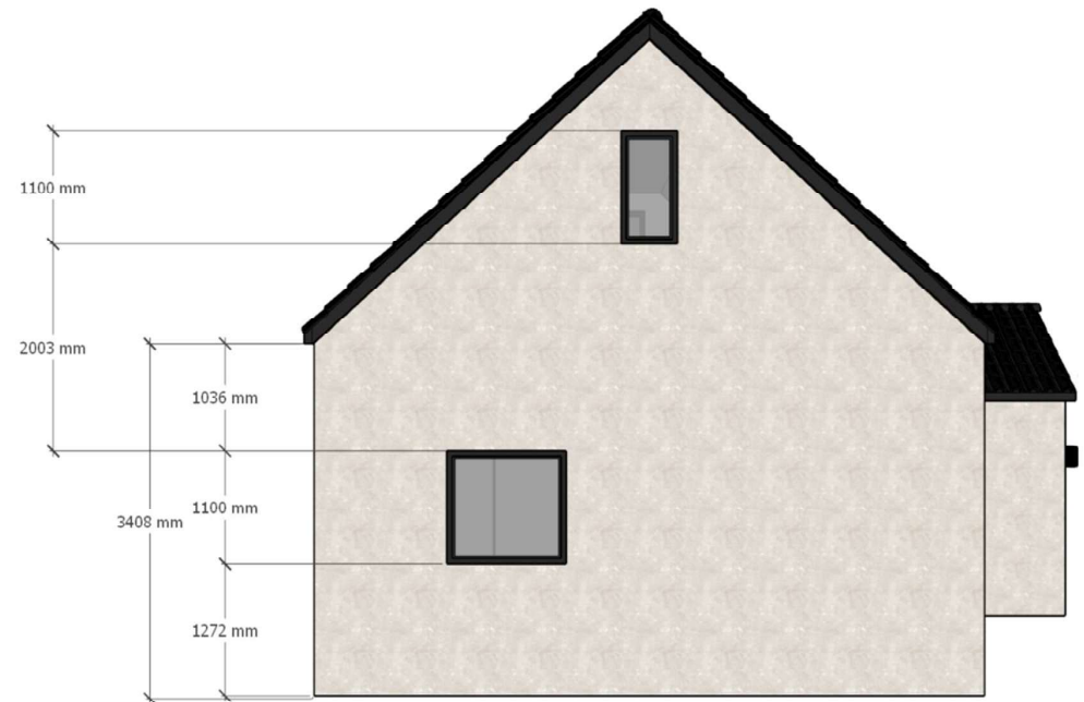
LHS ELEVATION
