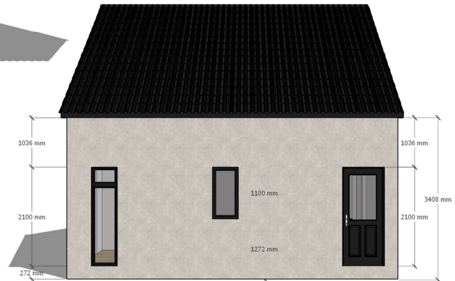
REAR ELEVATION
