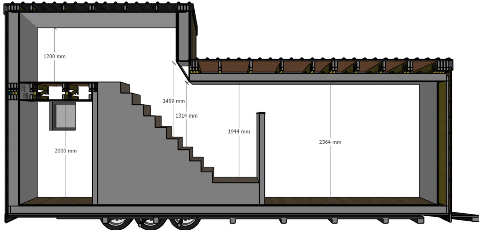
SECTION C-C
