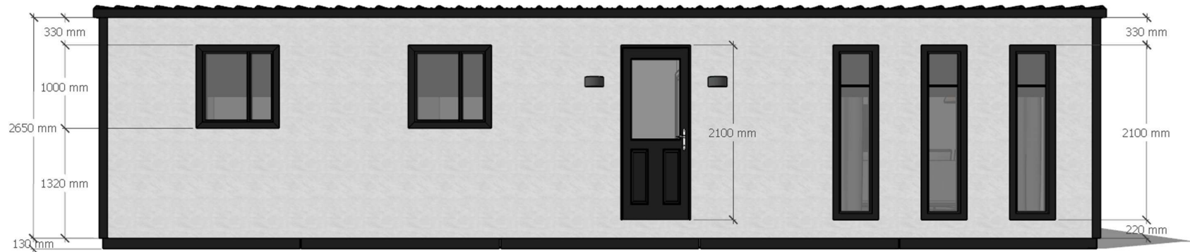
FRONT ELEVATION W/ DIMENSIONS
