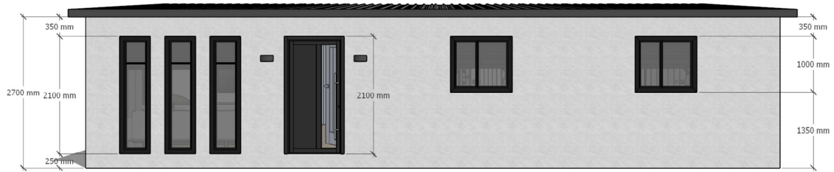
FRONT ELEVATION
