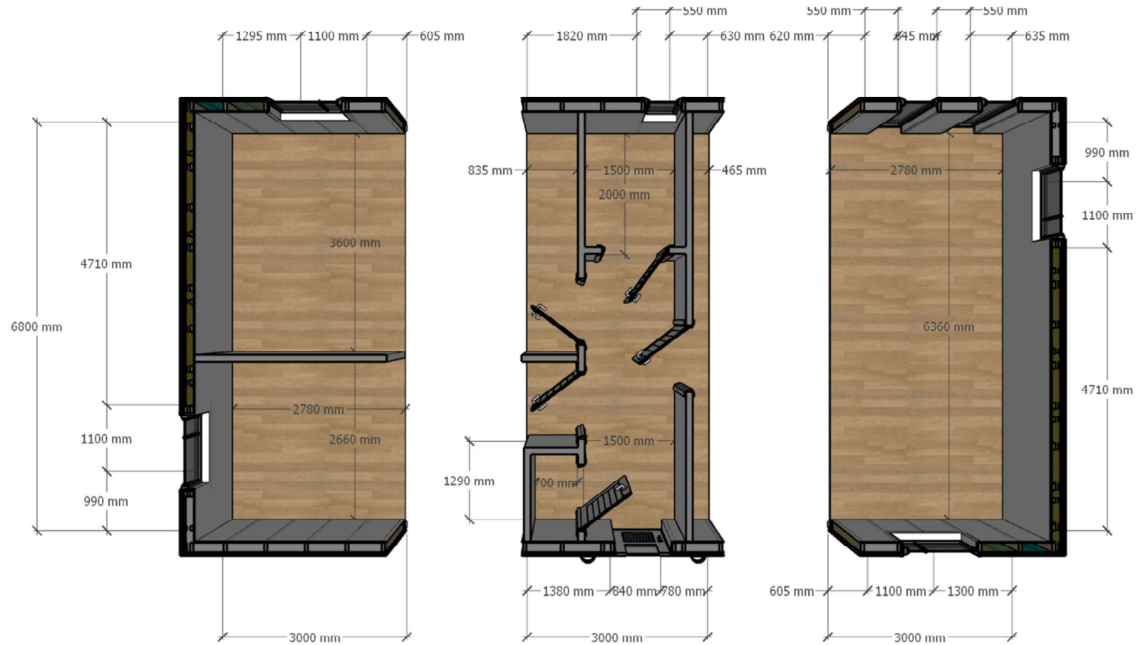
SECTION PLAN
