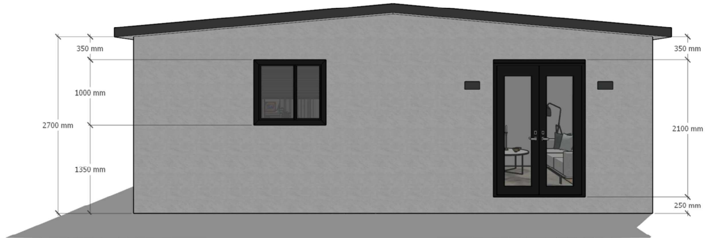
LHS ELEVATION
