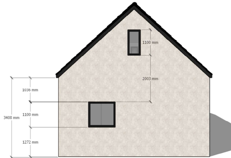
LHS ELEVATION
