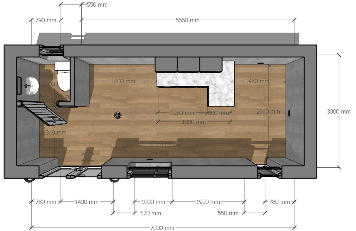
FLOOR PLAN 01 –LAYOUT
