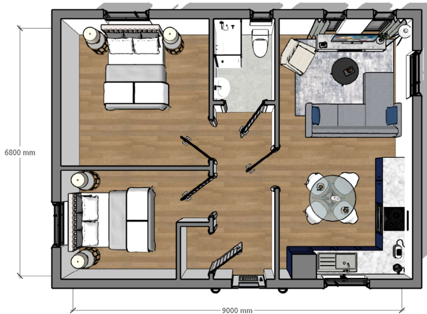
FLOOR PLAN - Example of furniture layout
