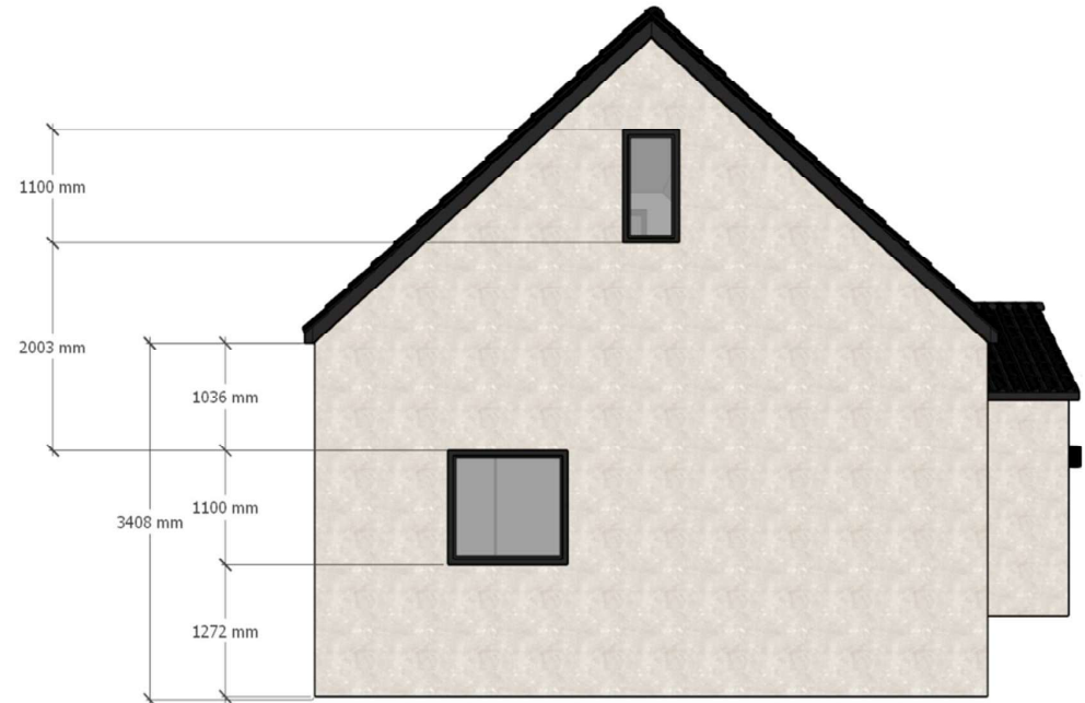
LHS ELEVATION
