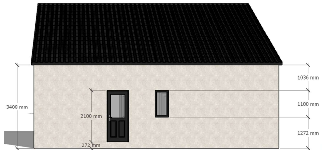
REAR ELEVATION
