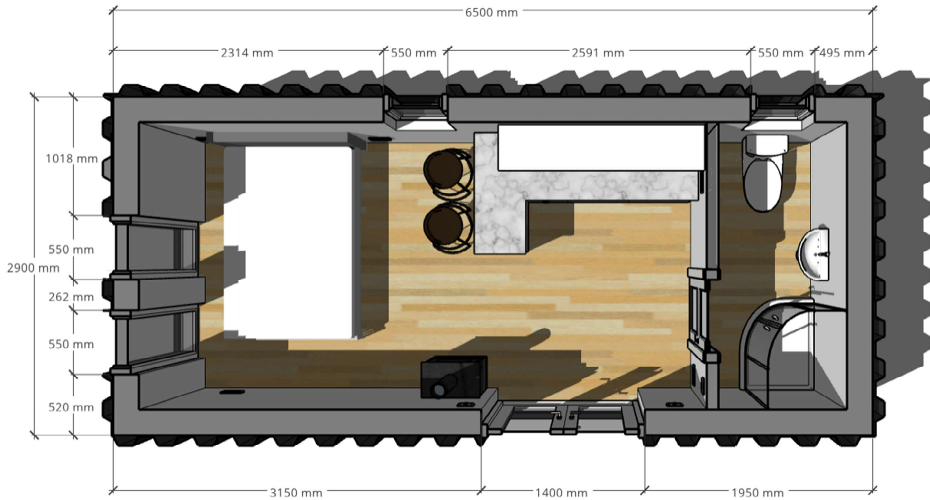
FLOOR PLAN 02
