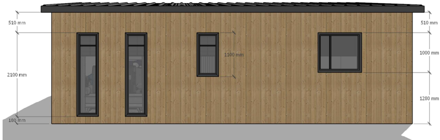
REAR ELEVATION
