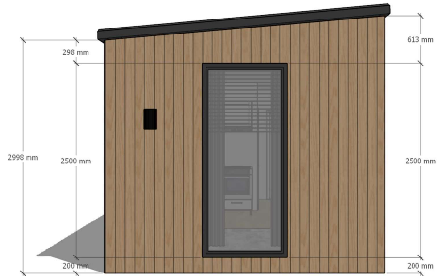
LHS ELEVATION
