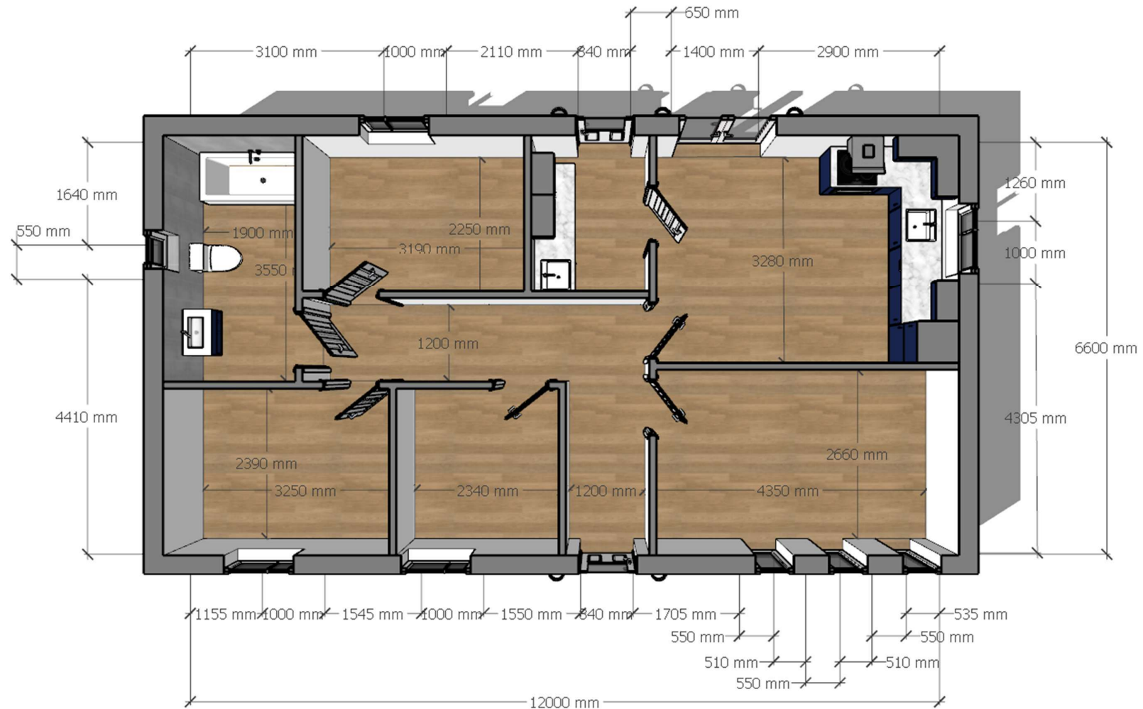
FLOOR PLAN 01 –LAYOUT
