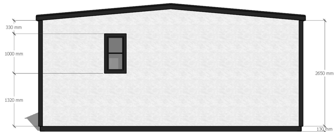
RHS ELEVATION W/ DIMENSIONS
