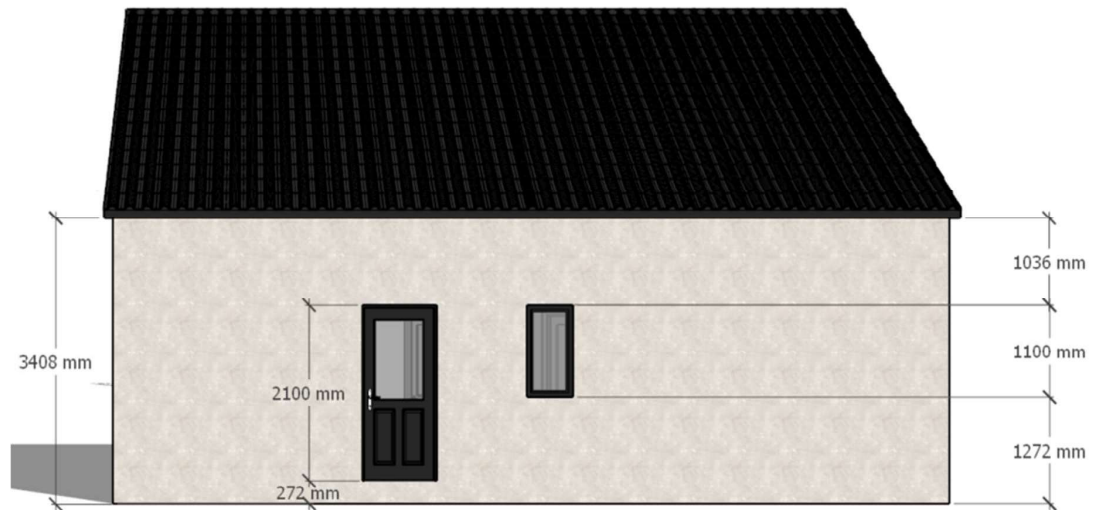
REAR ELEVATION
