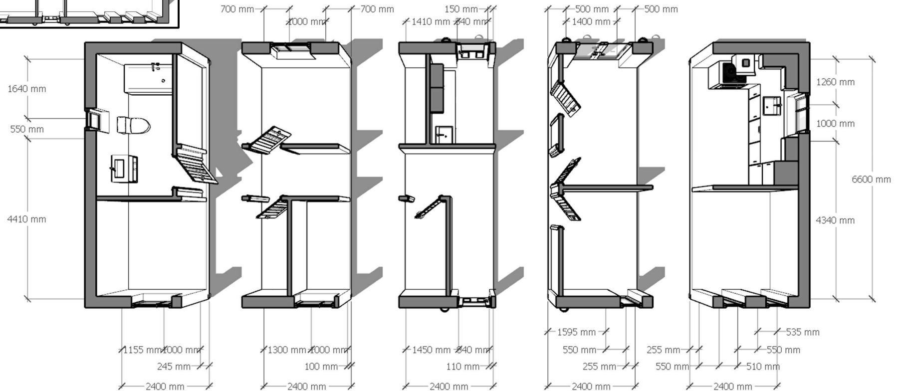
FLOOR PLAN 03 – MODULAR SECTIONS
