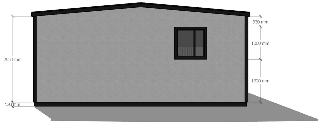
LHS ELEVATION W/ DIMENSIONS
