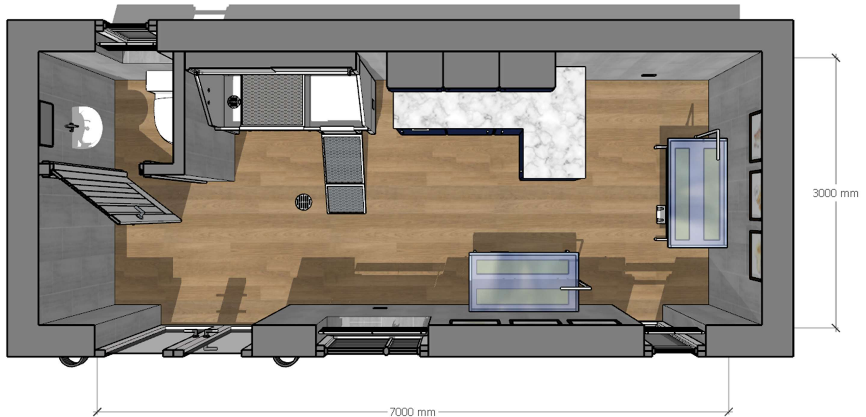
FLOOR PLAN 02 – FURNITURE LAYOUT (EXAMPLE ONLY)
