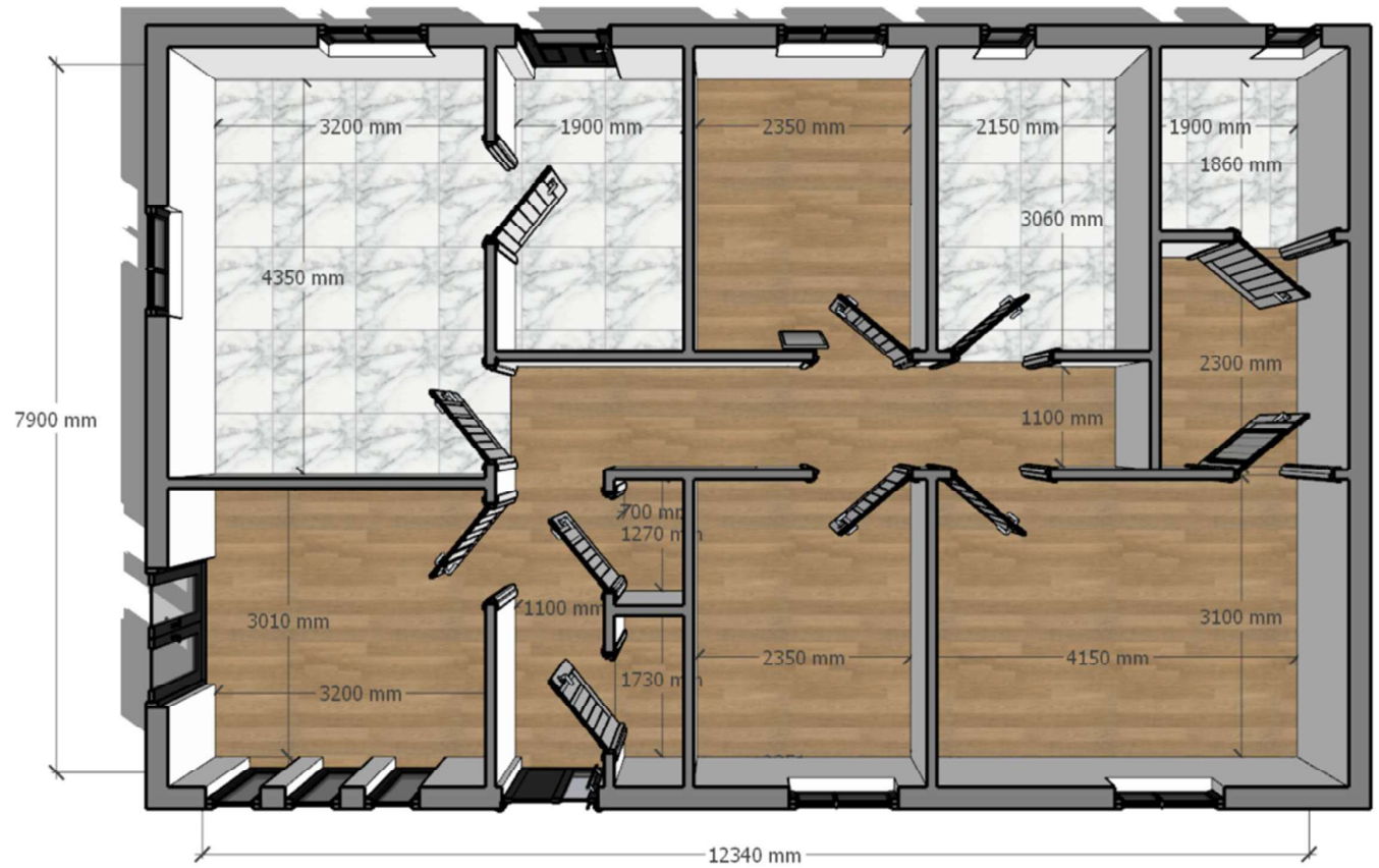
FLOOR PLAN 01
