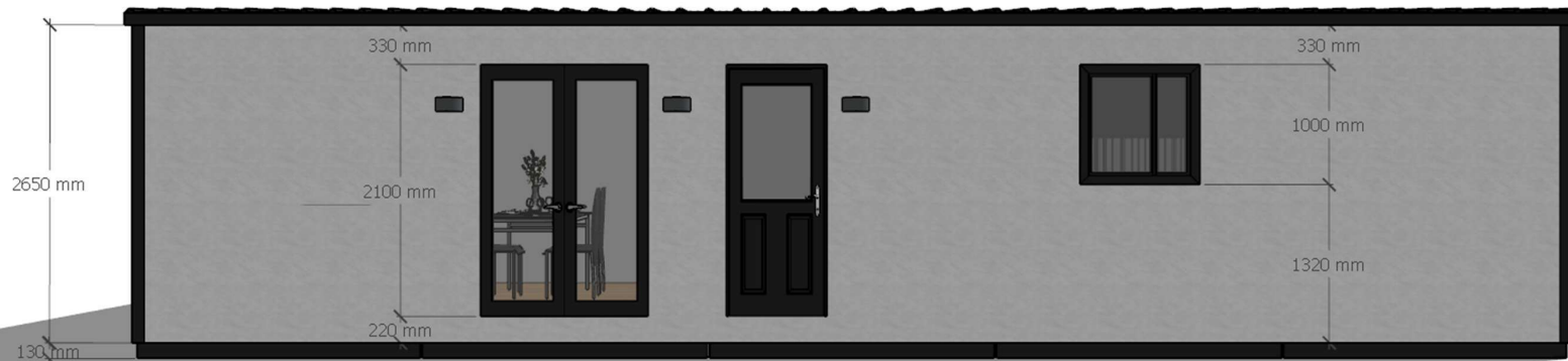
REAR ELEVATION W/ DIMENSIONS
