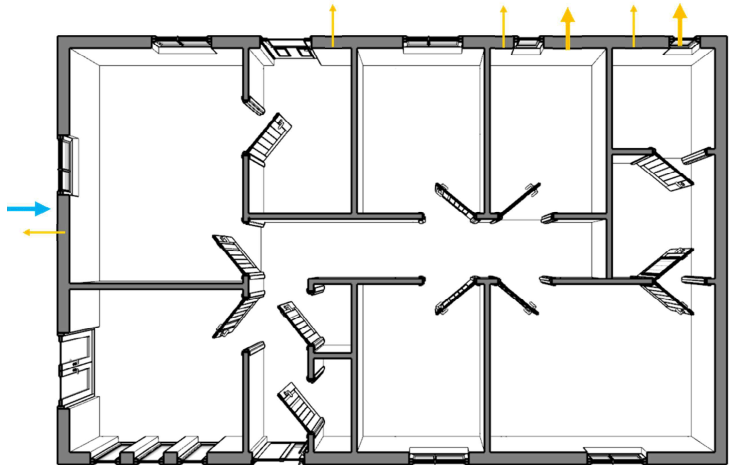
PLUMBING SERVICES LAYOUT
