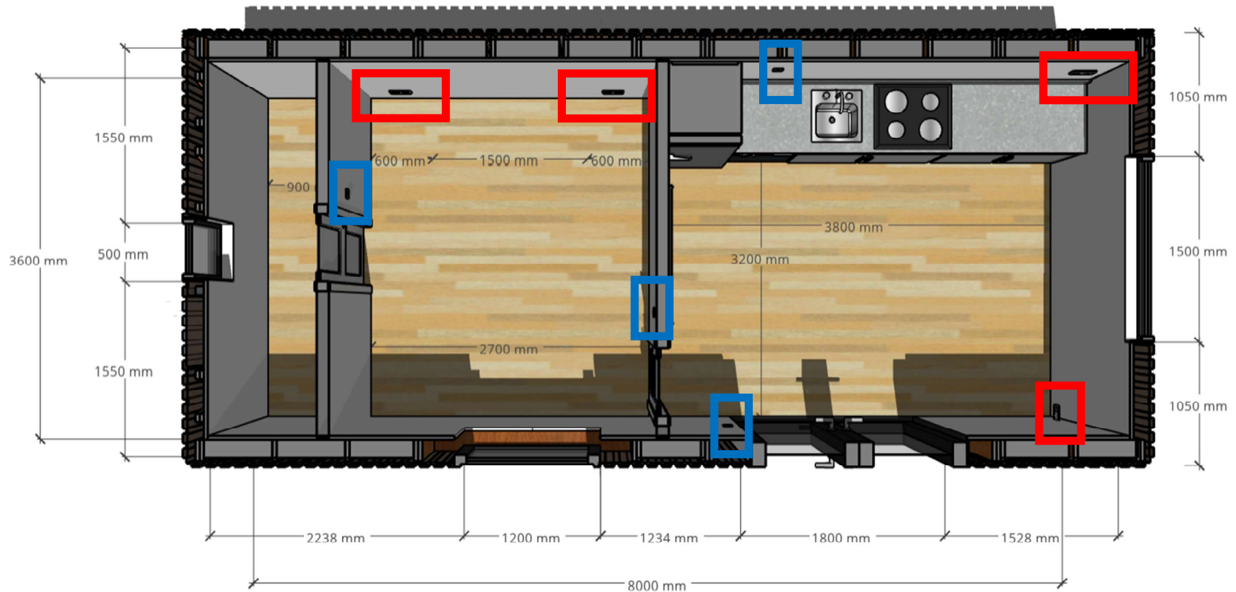
FLOOR PLAN 01
