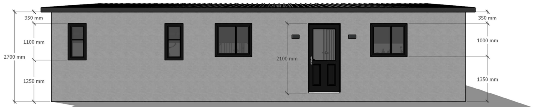
REAR ELEVATION
