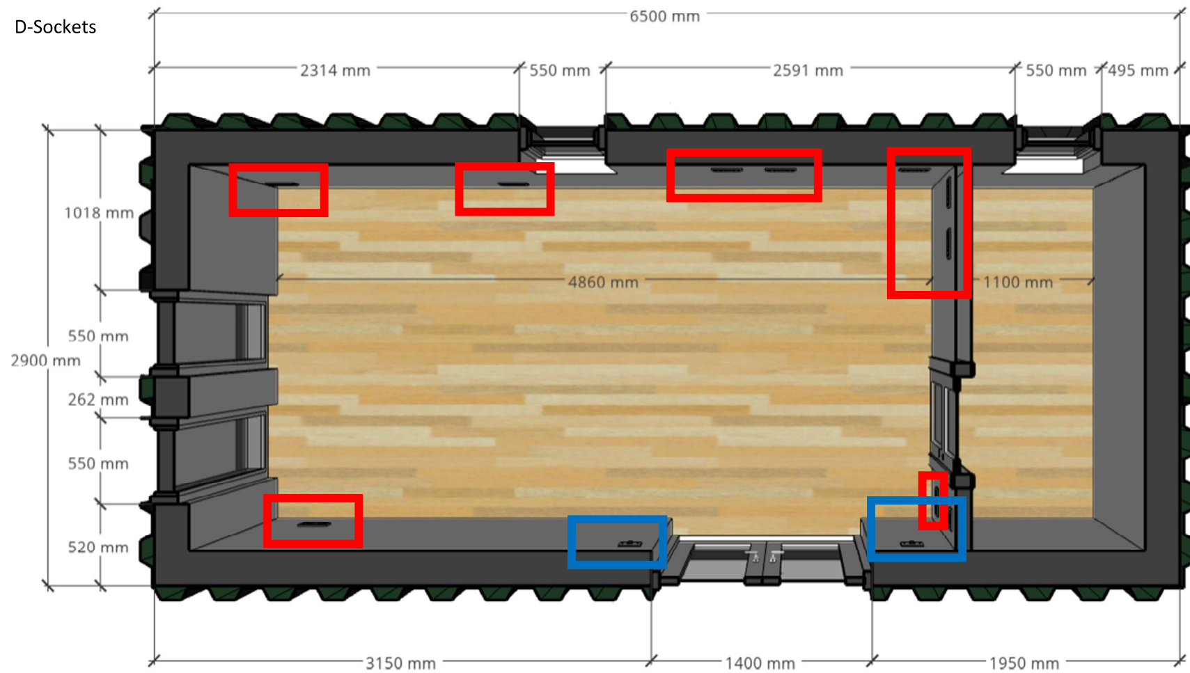
FLOOR PLAN 01
