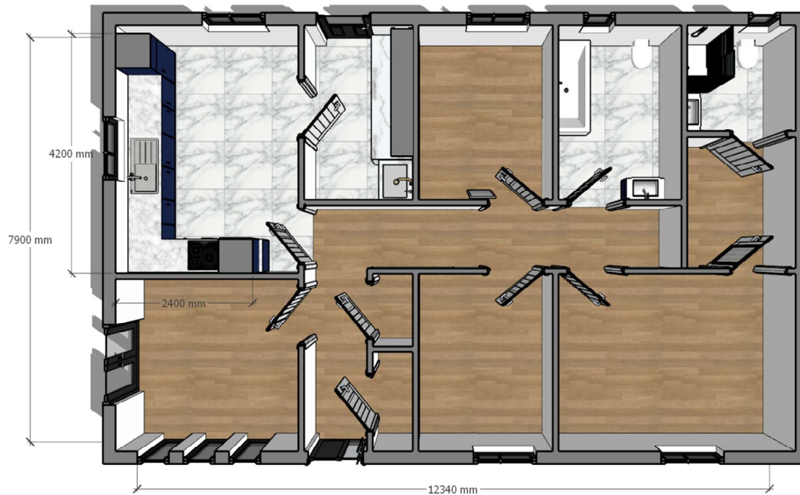
FLOOR PLAN 02
