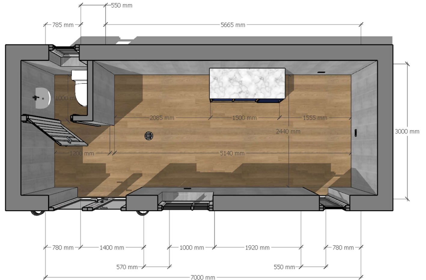
FLOOR PLAN 01 –LAYOUT
