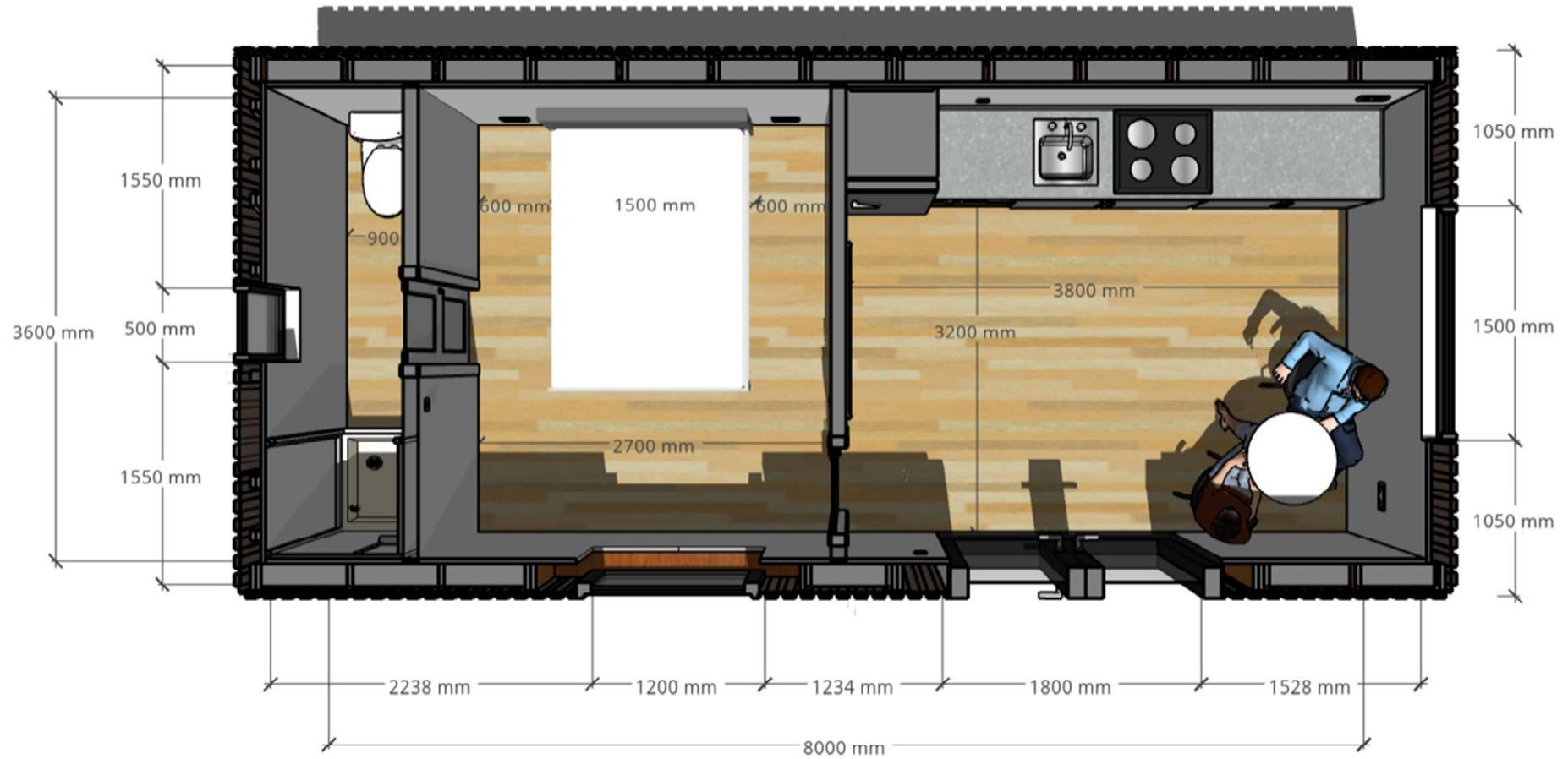
FLOOR PLAN 02
